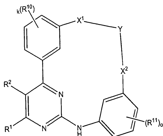
Formula (X)
