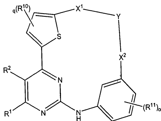
Formula (XI)
