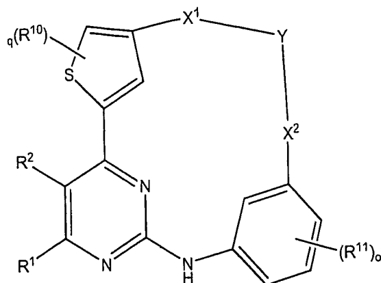
Formula (XVII)
