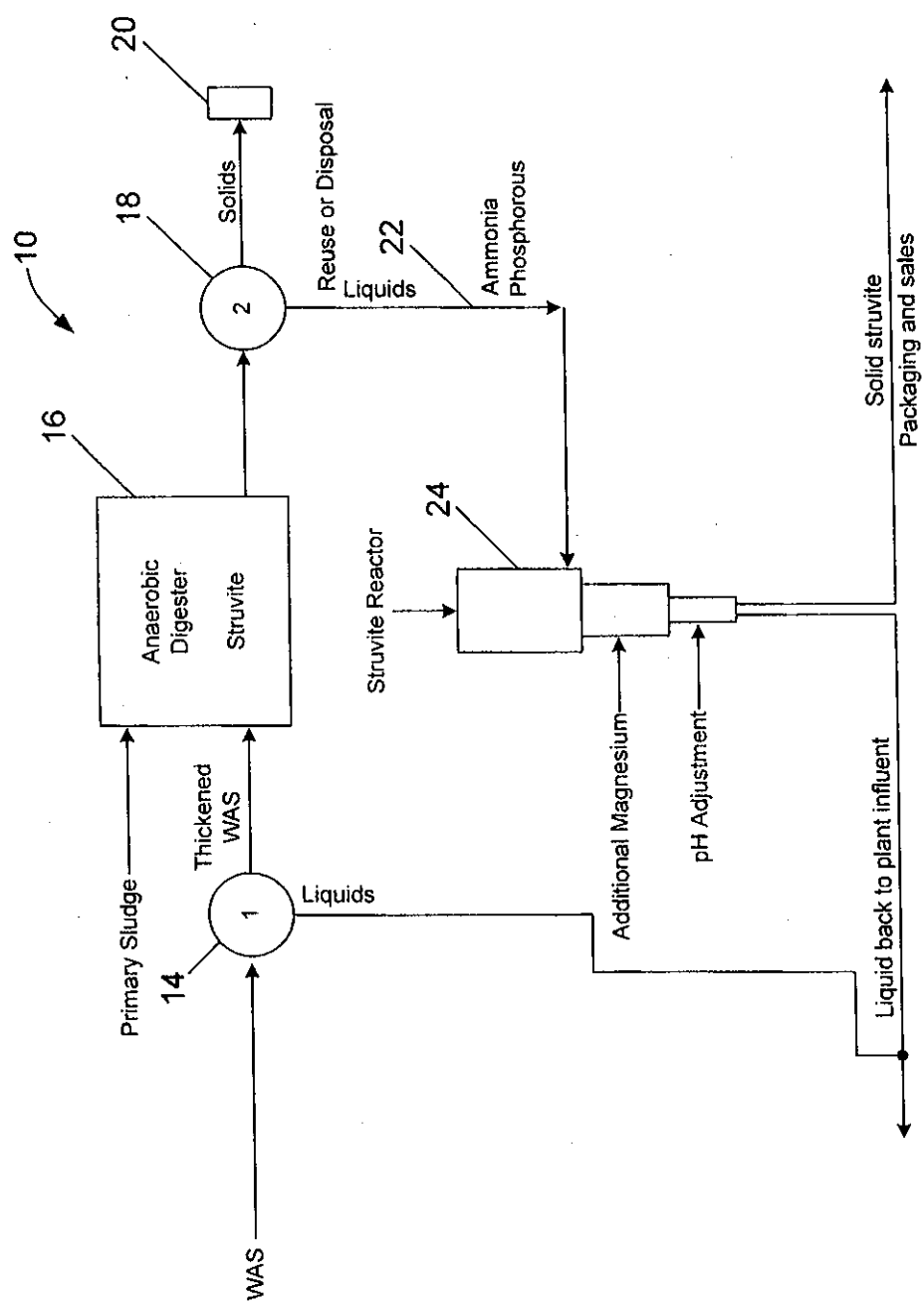
Figure 1 (Prior Art)
