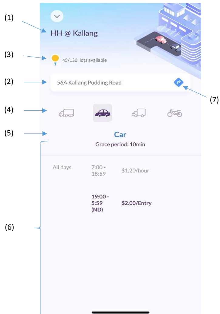
Figure 2. More Complete Carpark Information
