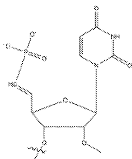
5' vinylphosphonate 2' O Methyl Uridine
