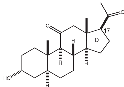
Compound A
