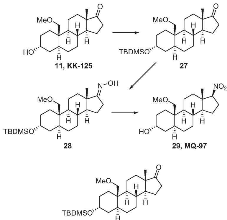
Scheme 8
