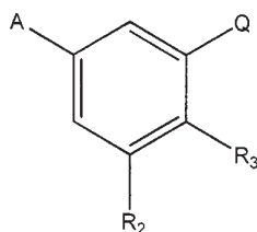
Formula I.1
