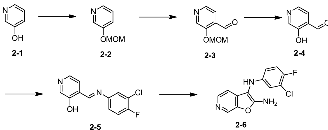
Scheme 2B
