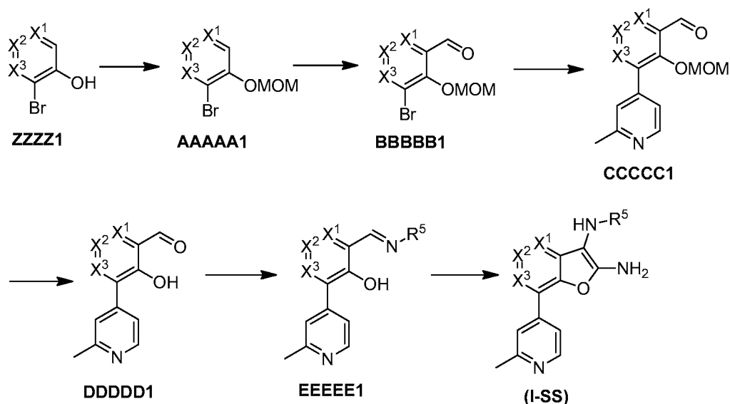
Scheme 23
