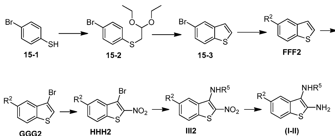
Scheme 15A
