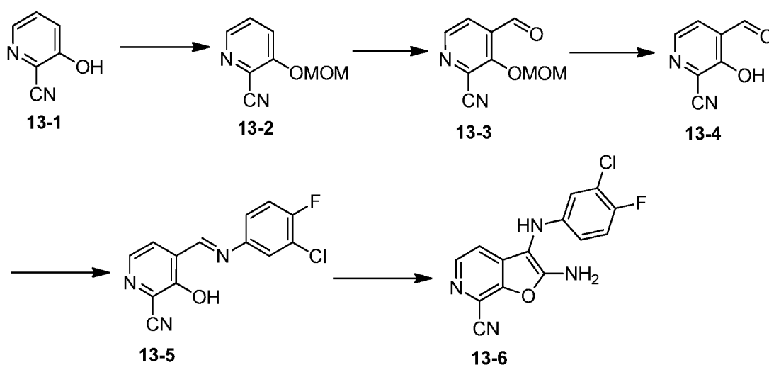
Scheme 13B
