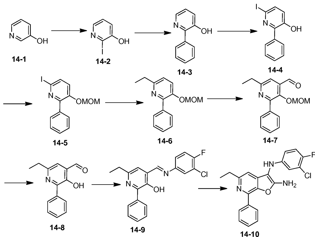
Scheme 14B
