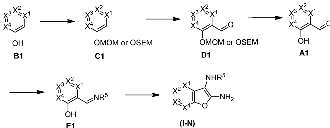
Scheme 6
