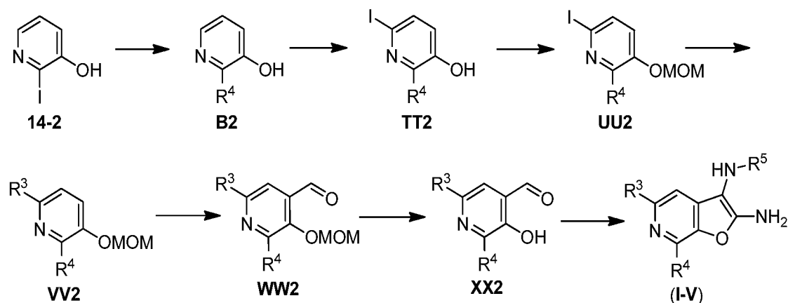
Scheme 28A
