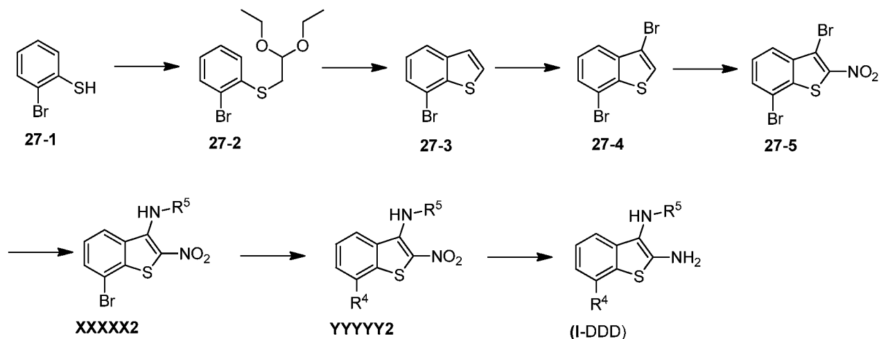
Scheme 27A
