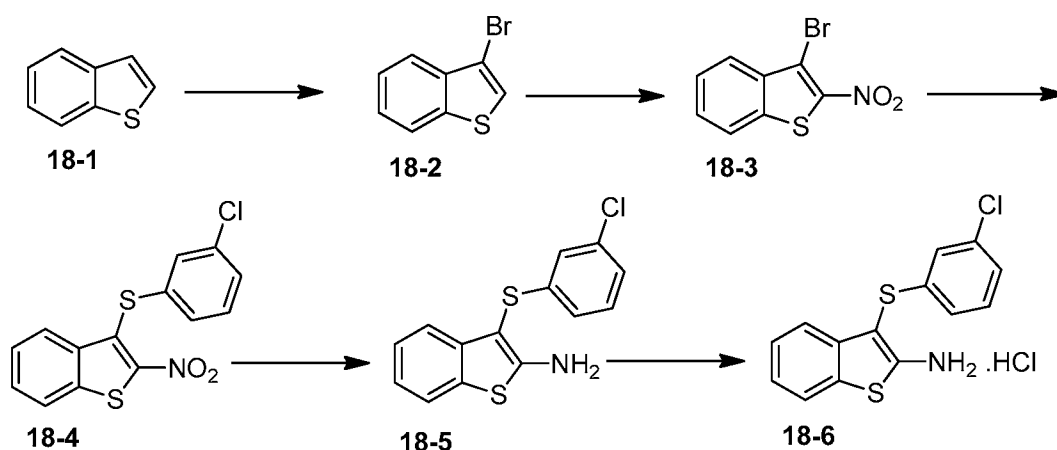
Scheme 18B
