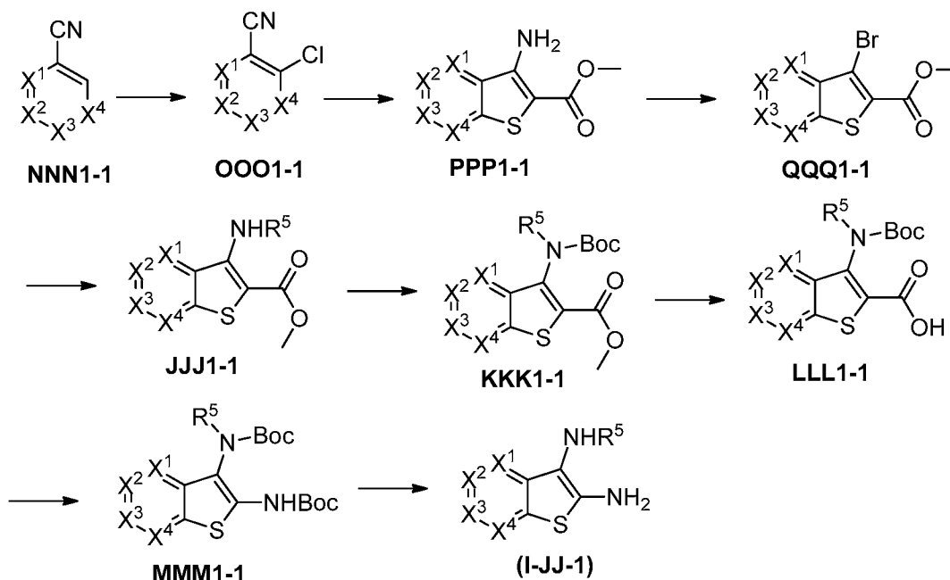
Scheme 16
