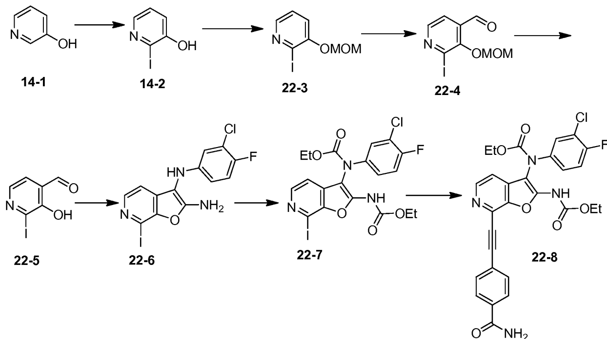
Scheme 22B
