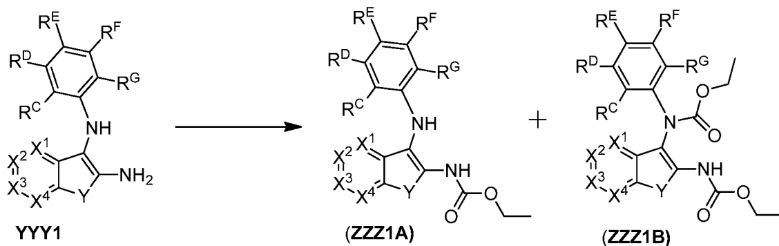
Scheme 20
