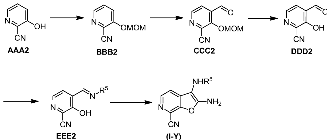
Scheme 13A2
