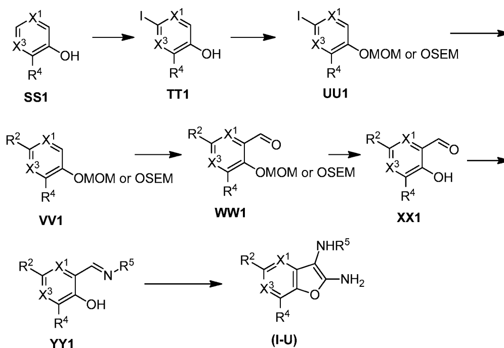
Scheme 11
