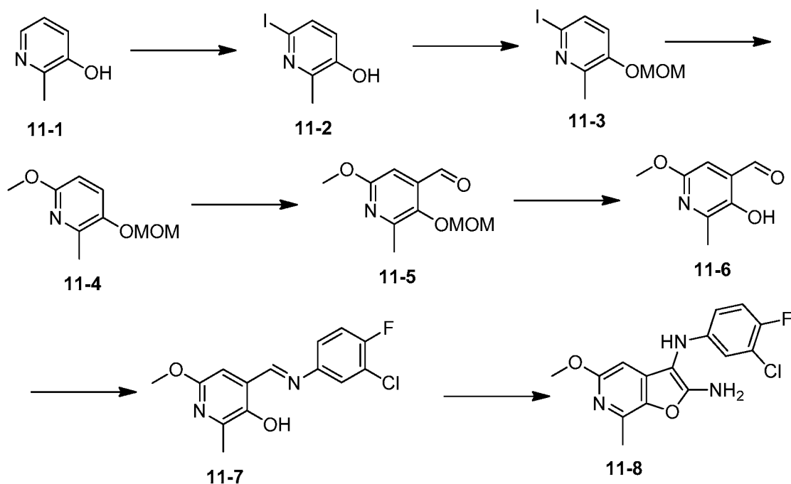
Scheme 11B
