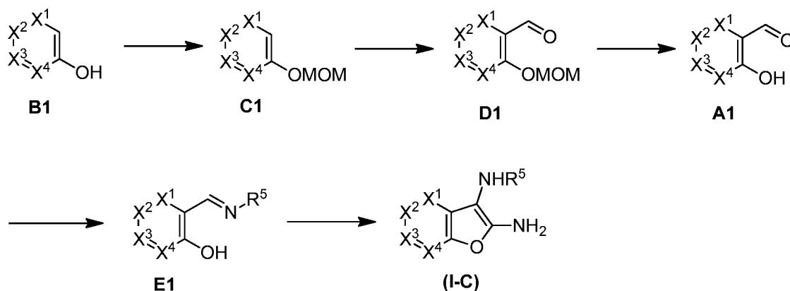
Scheme 4
