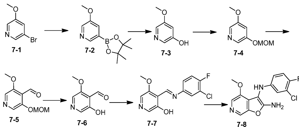
Scheme 7B
