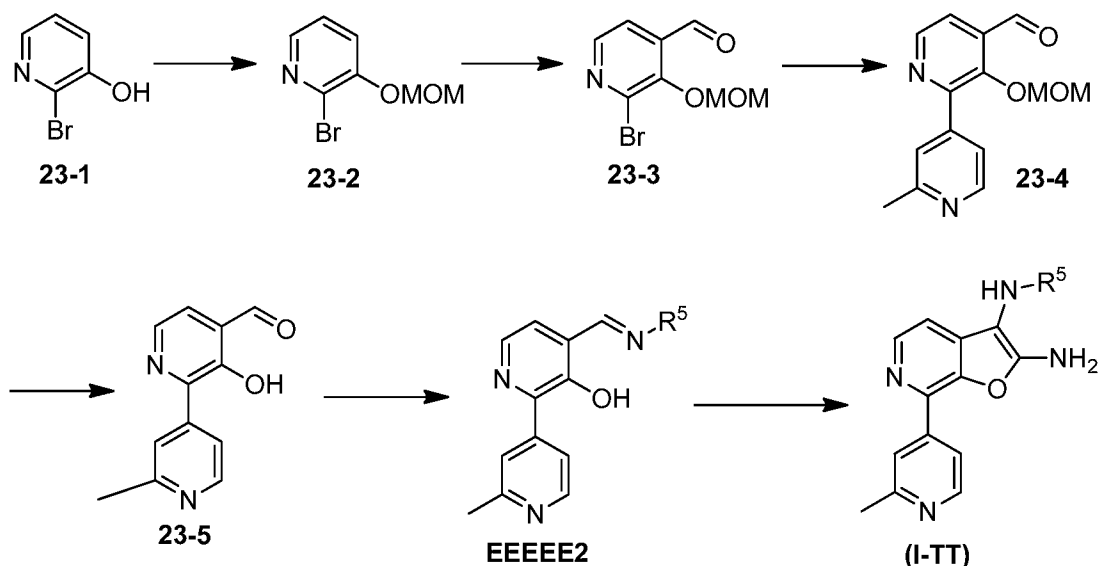
Scheme 23A
