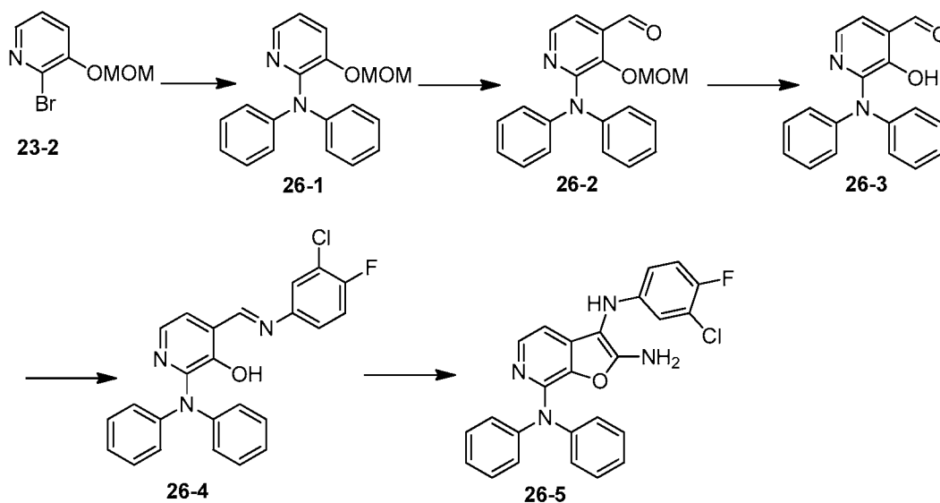
Scheme 26B
