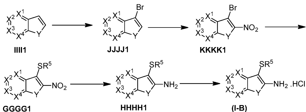
Scheme 18
