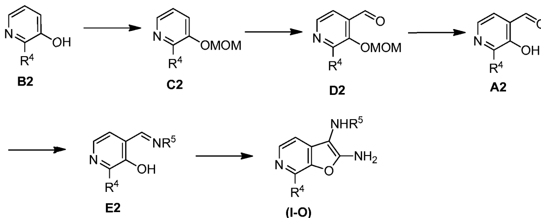
Scheme 6A
