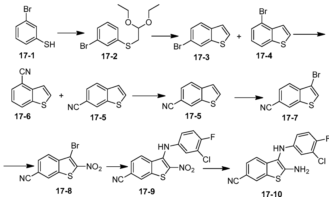
Scheme 17B
