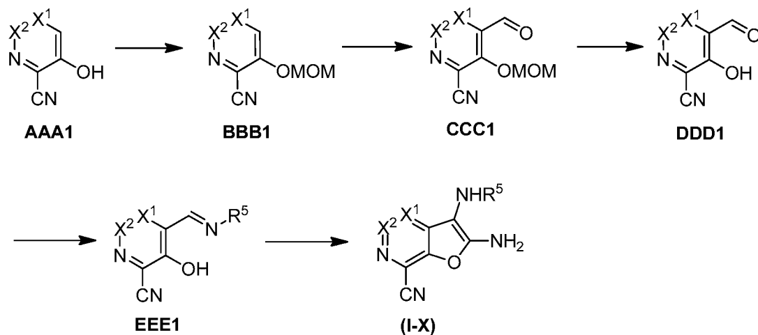
Scheme 13A1
