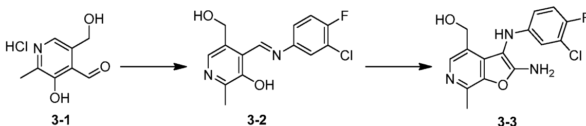
Scheme 3B
