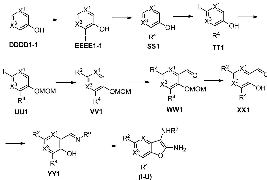
Scheme 14
