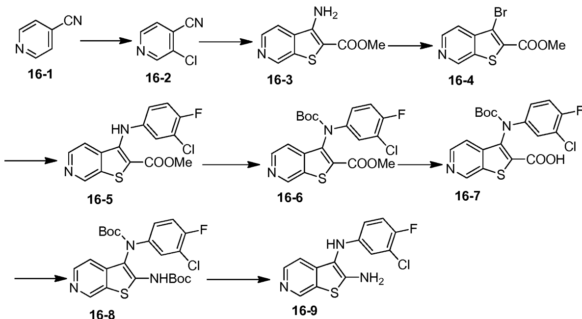
Scheme 16B
