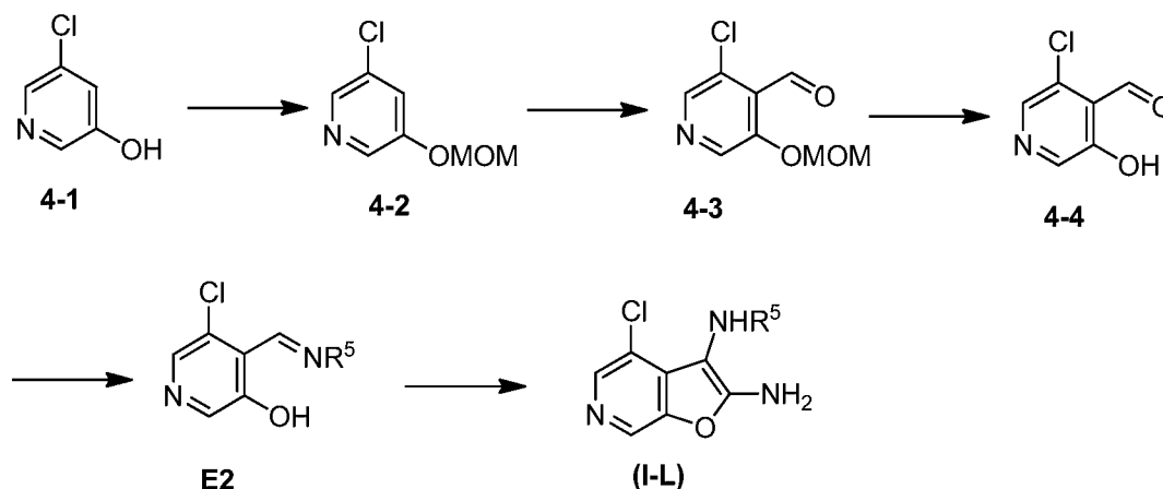
Scheme 4A
