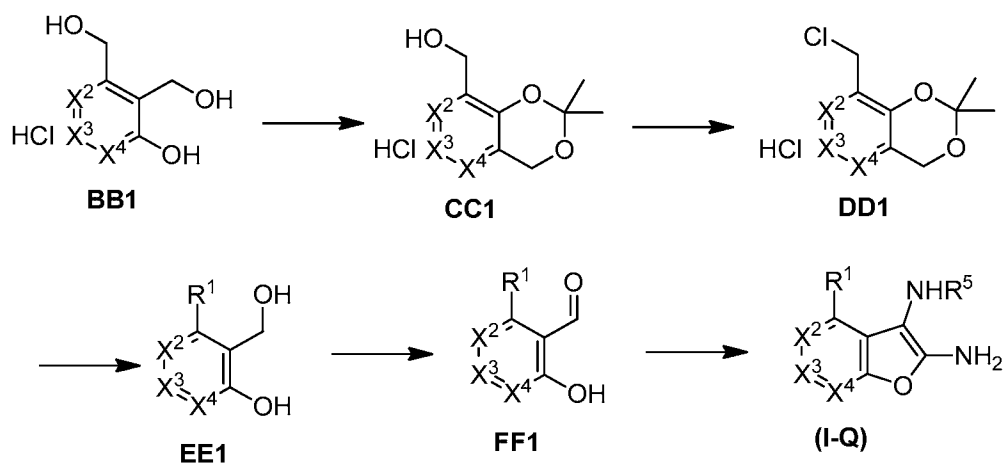
Scheme 8
