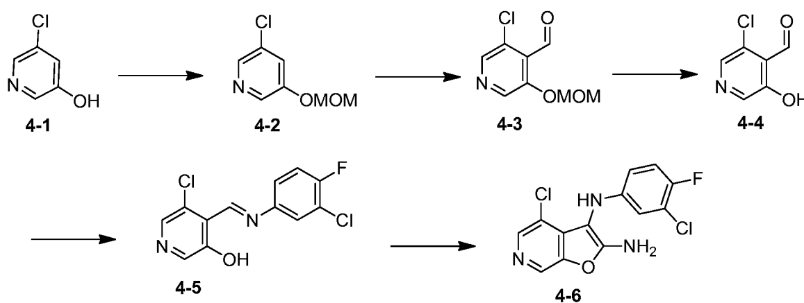
Scheme 4B
