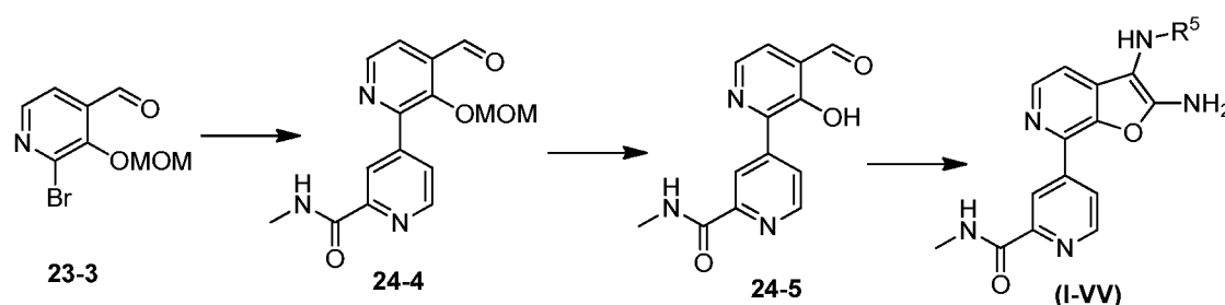
Scheme 24A
