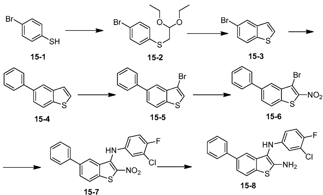
Scheme 15B
