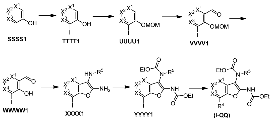
Scheme 22
