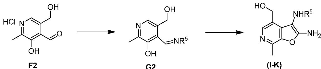
Scheme 3A
