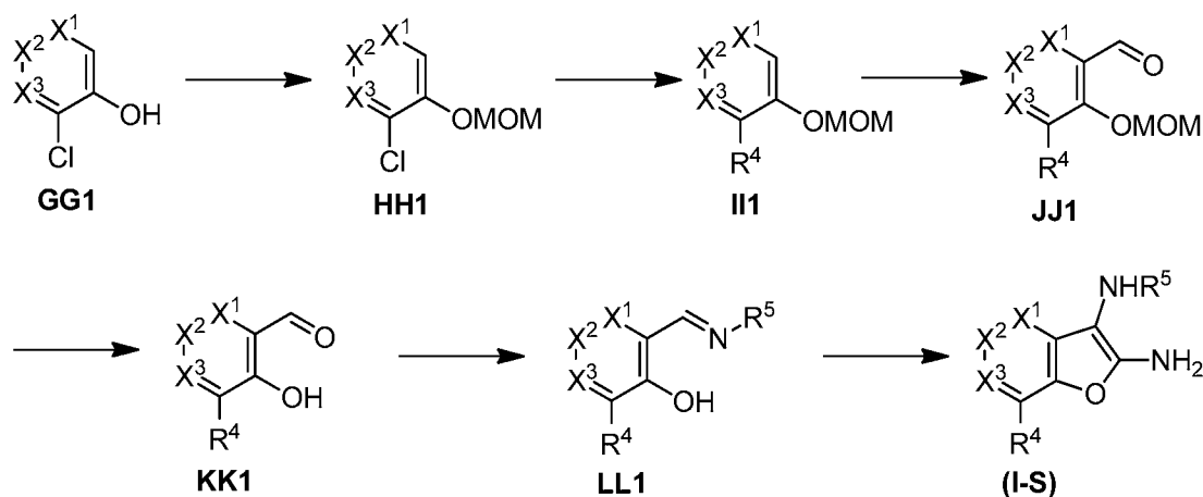
Scheme 9
