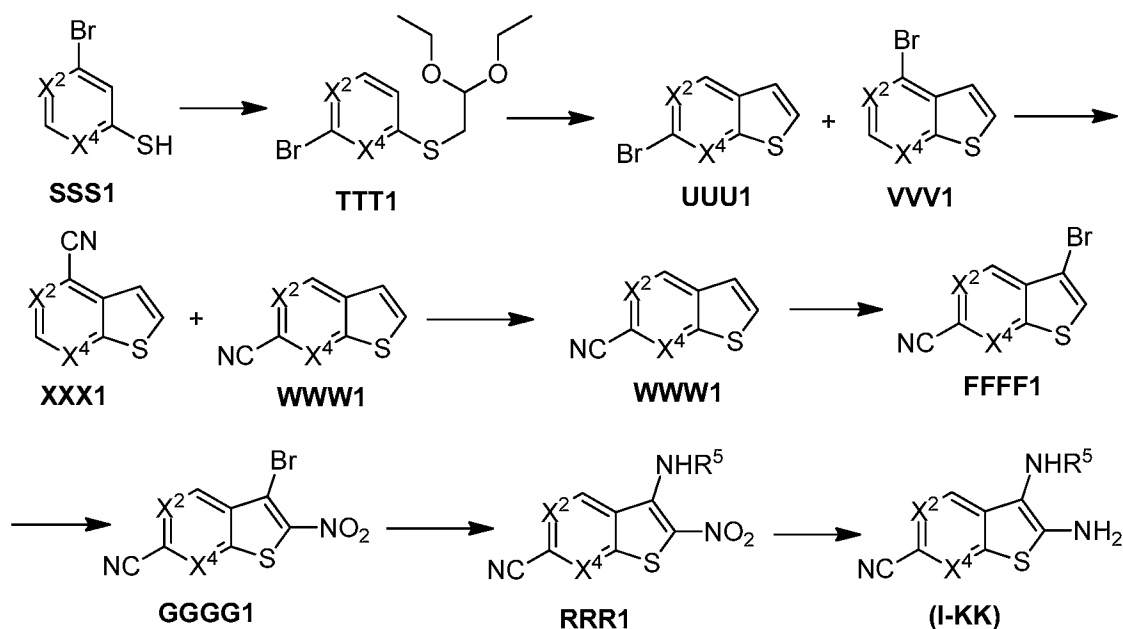
Scheme 17
