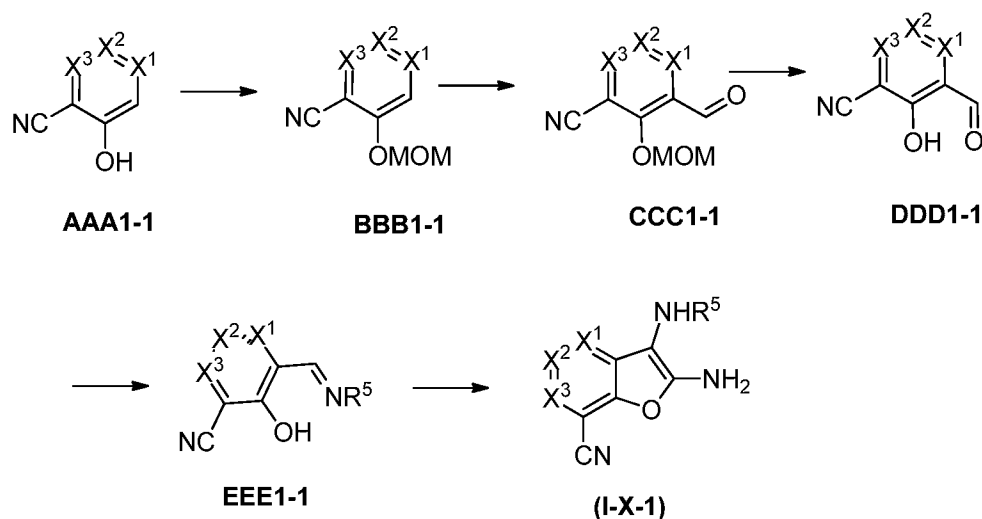
Scheme 13
