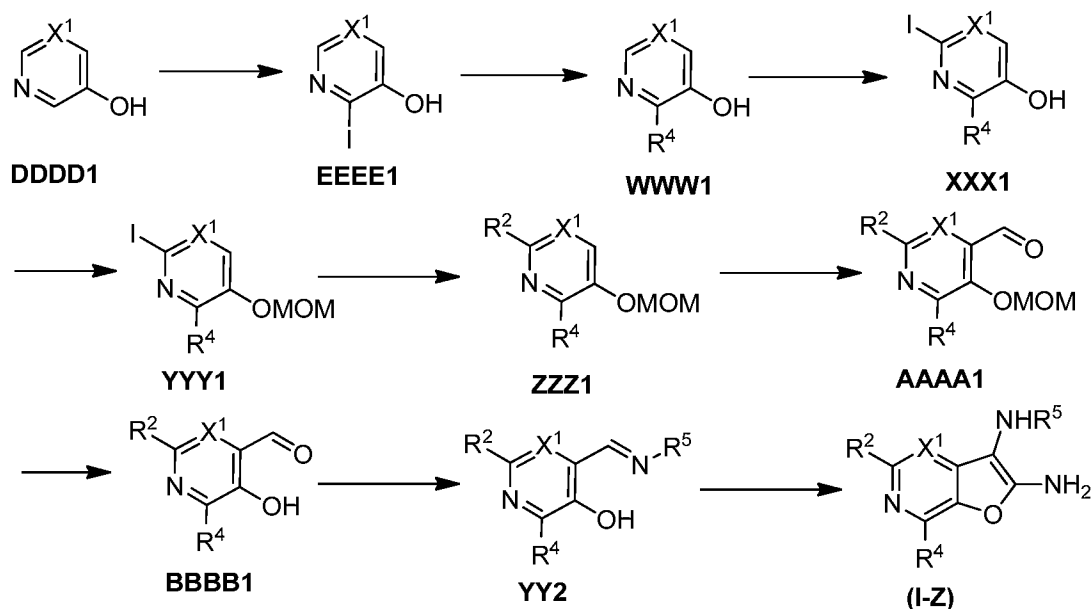
Scheme 14A1
