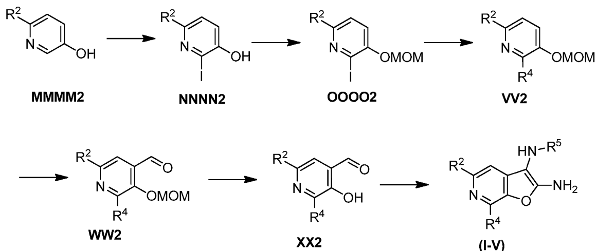
Scheme 21A
