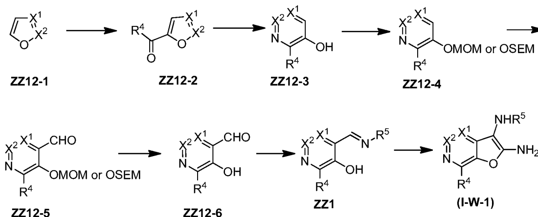
Scheme 12
