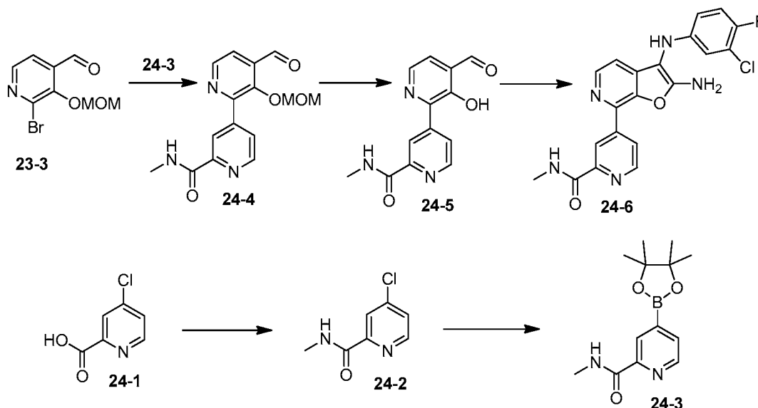
Scheme 24B
