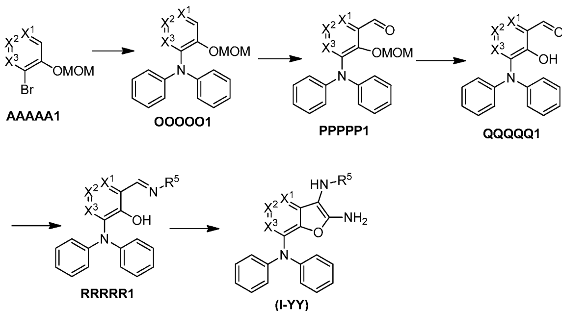
Scheme 26
