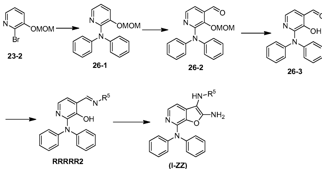
Scheme 26A
