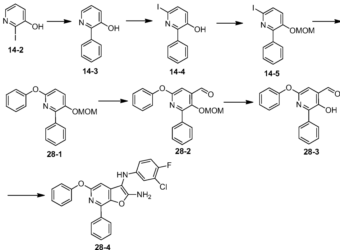
Scheme 28B
