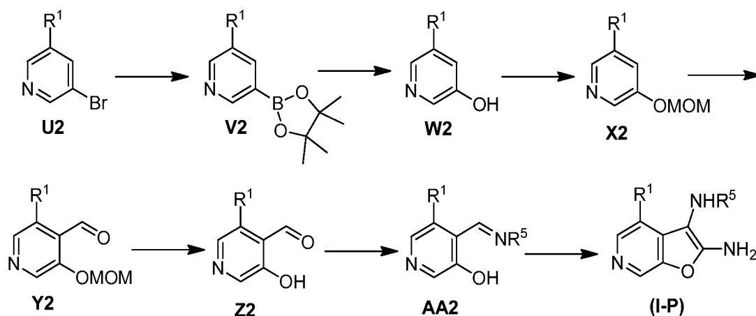
Scheme 7A
