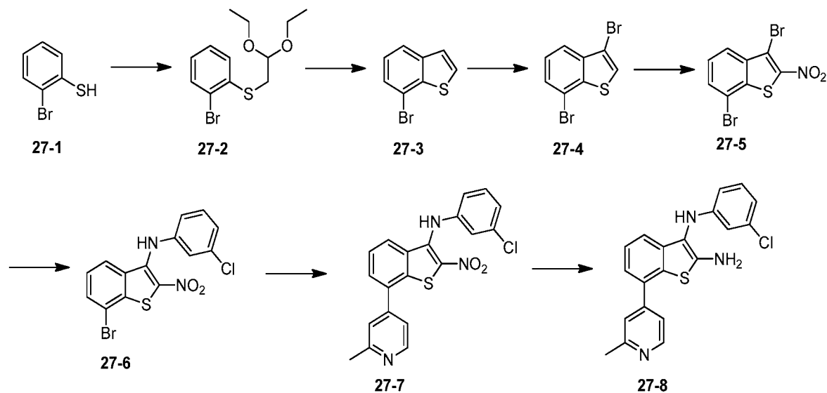
Scheme 27B
