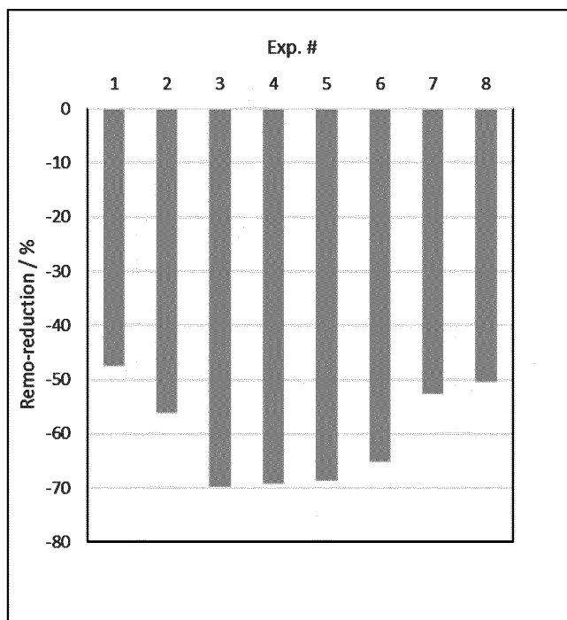
Figure 3: Reduction of the residual methyl methacrylate content in experiments 1 to 8.
