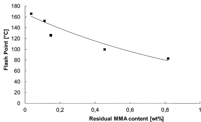
Figure 4: Correlation of the flash point of the polymers with an increase in residual MMA concentration.
