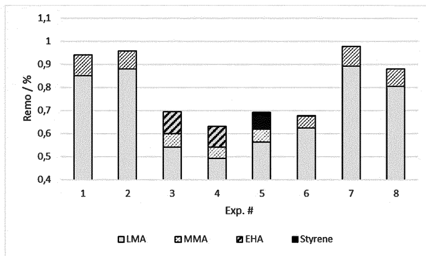
Figure 1: Residual monomer contents in the products of experiments 1 to 8.
