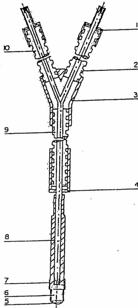
Figure1: Configuration of the Fiber Optic Temperature Switching Immersion Probe
