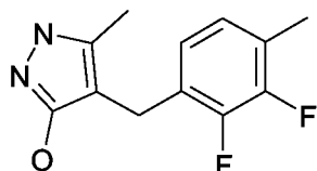
(13) 4-(2,3-Difluoro-4-methyl-benzyl)-5-methyl-1H-pyrazol-3-ol
