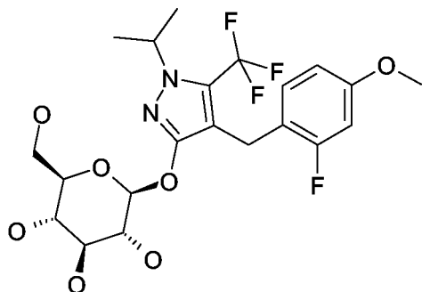
(17) 4-(2-fluoro-4-methoxy-benzyl)-1-isopropyl-5-trifluoromethyl-3-β-D-glucopyranos-1-yloxy-1H-pyrazole
