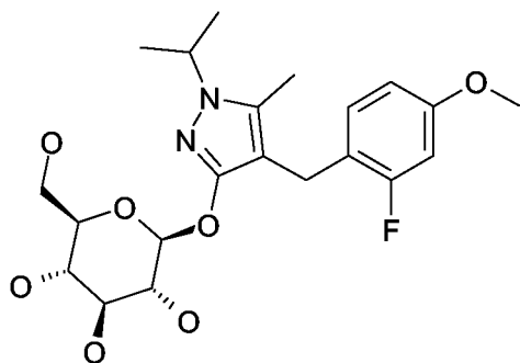
(17) 4-(2-fluoro-4-methoxy-benzyl)-1-isopropyl-5-trifluoromethyl-3-β-D-glucopyranos-1-yloxy-1H-pyrazole
