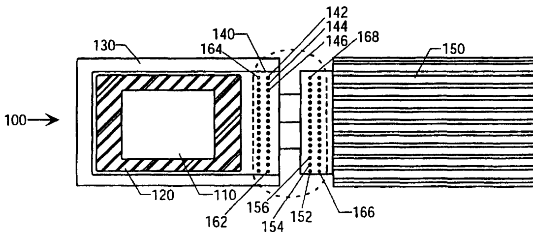
TOP VIEW (UNASSEMBLED)
