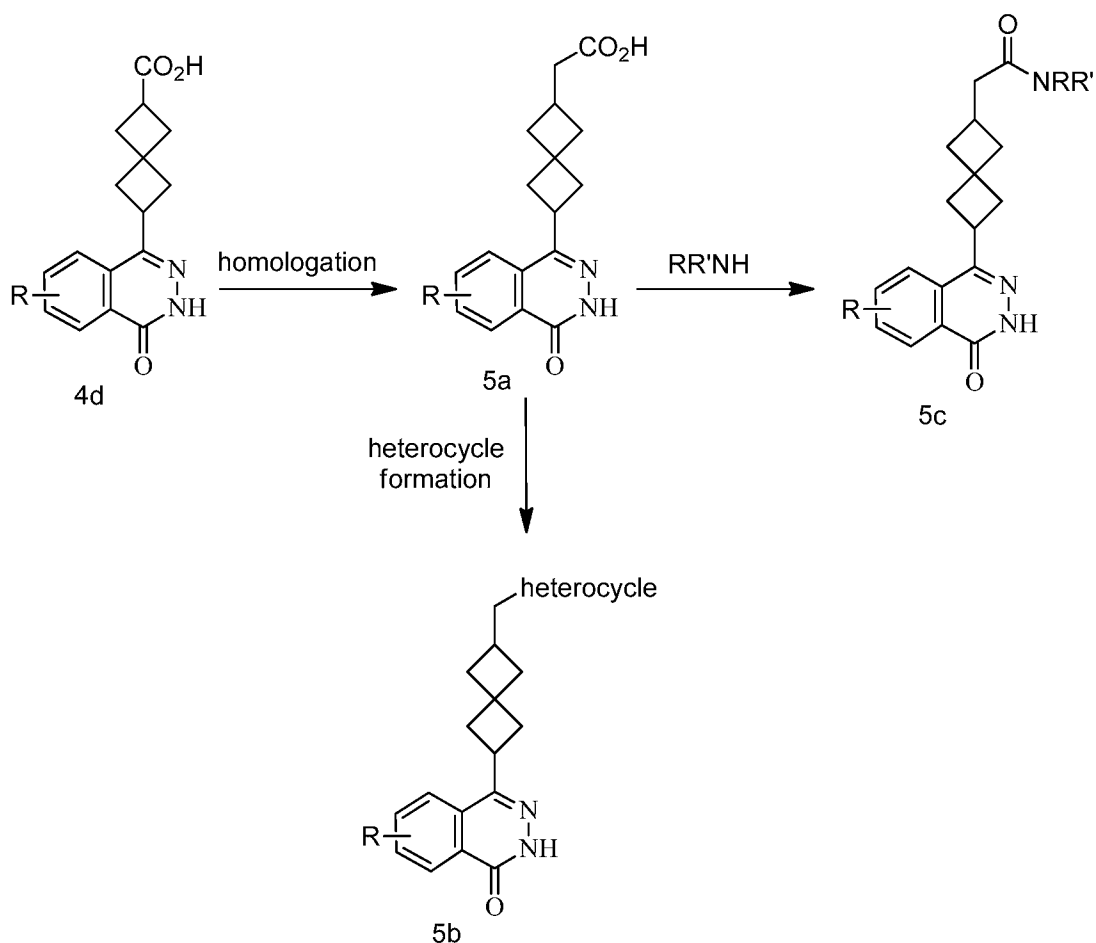
Scheme 5
