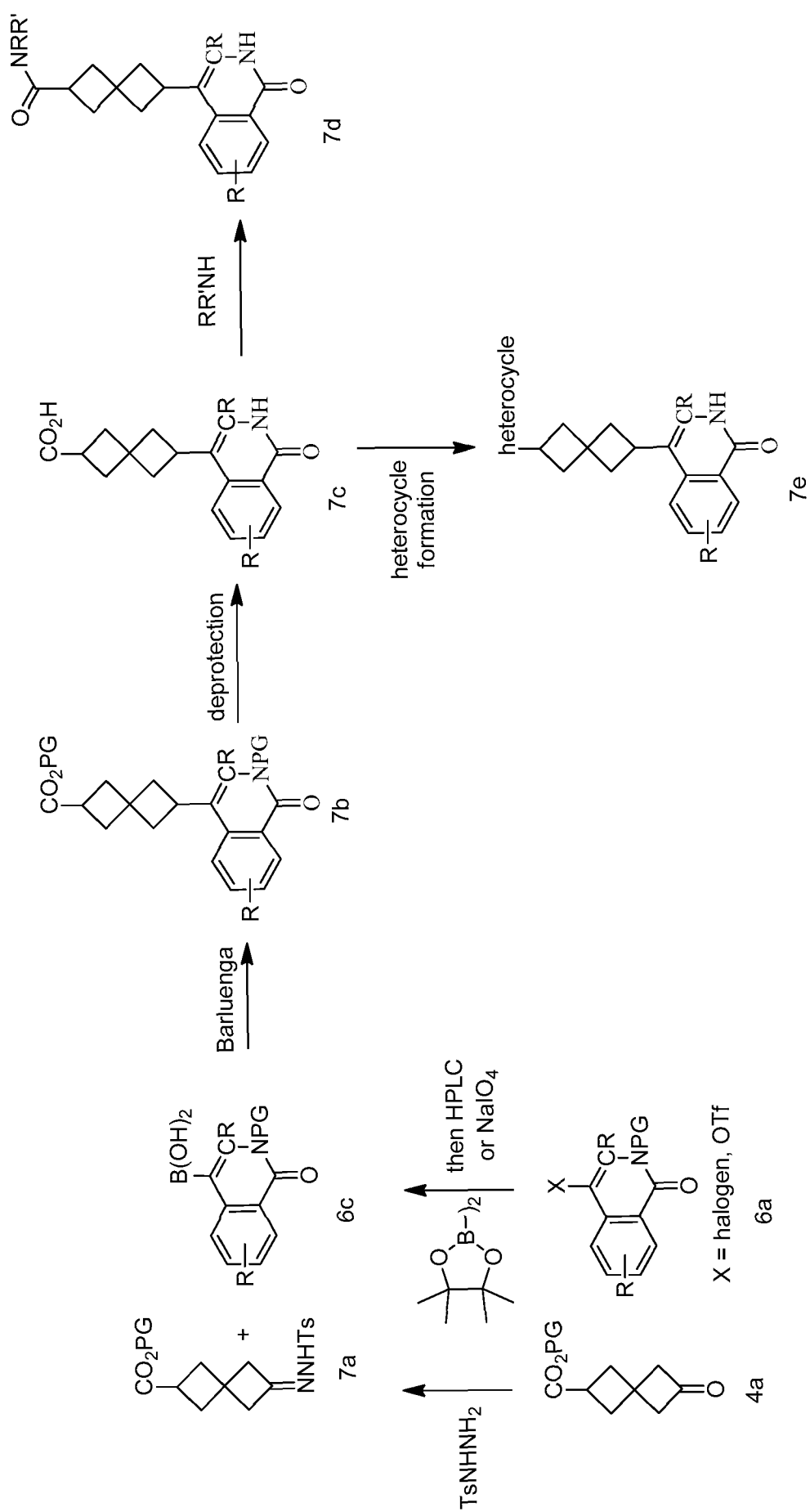
Scheme 7
