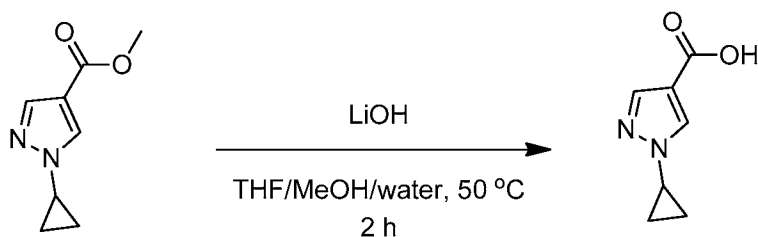
Intermediate 13:
