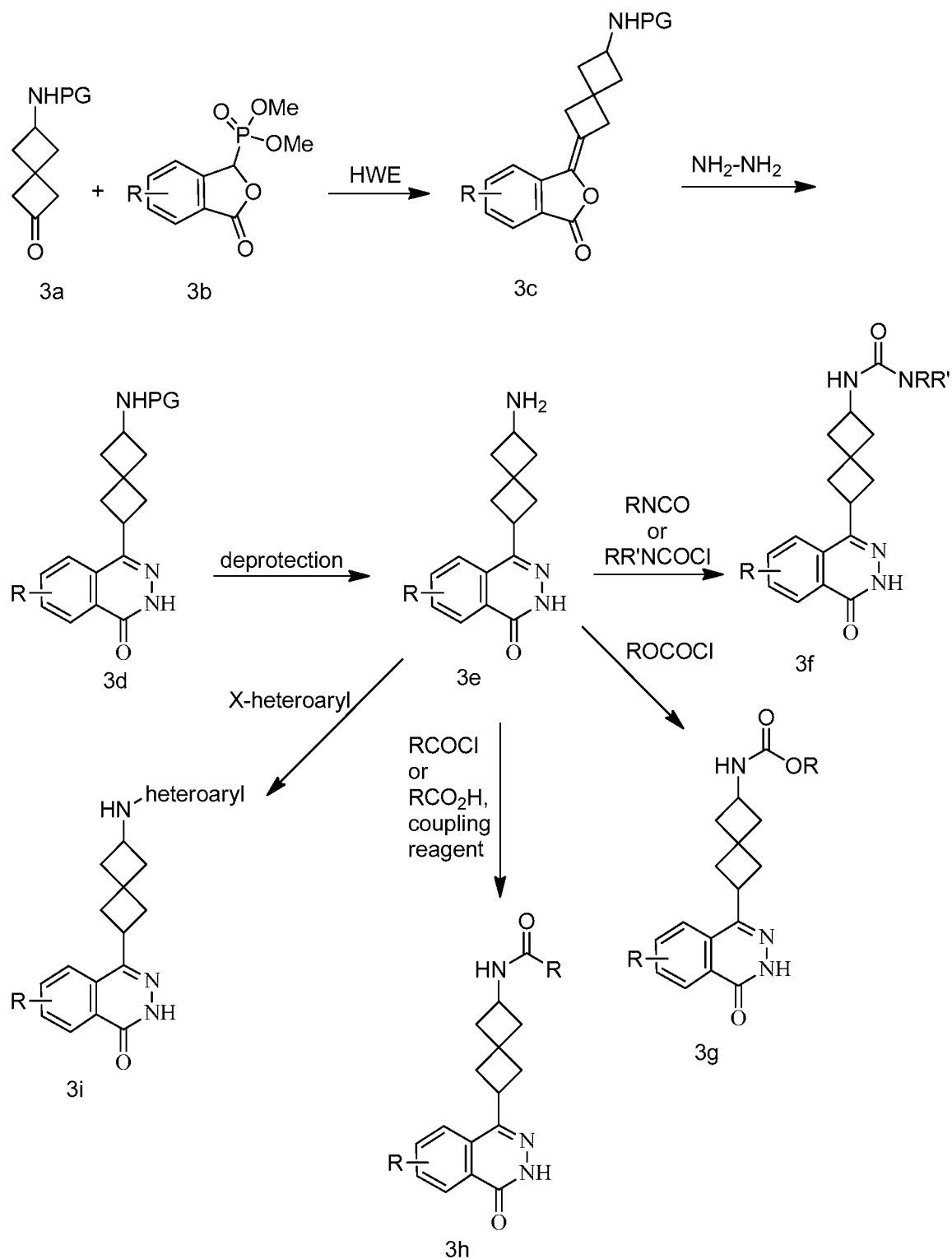
Scheme 3
