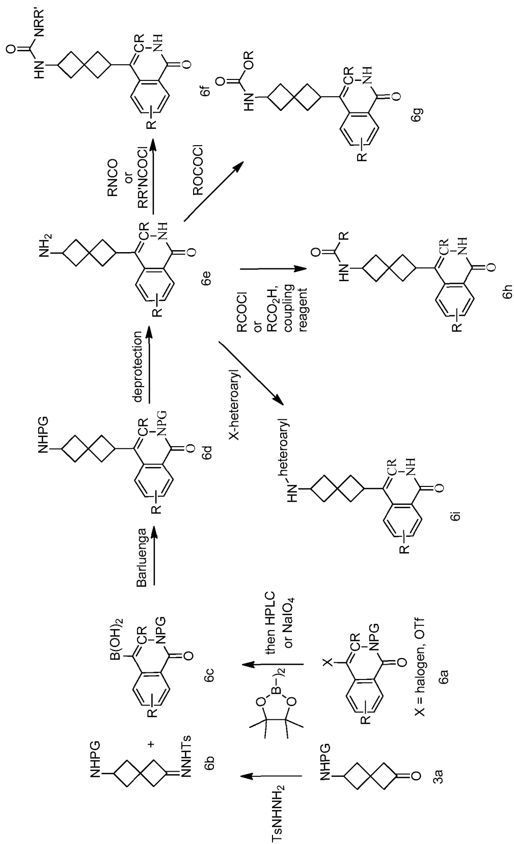
Scheme 6
