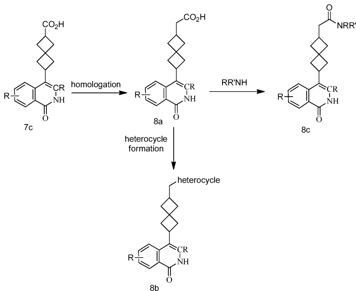
Scheme 8
