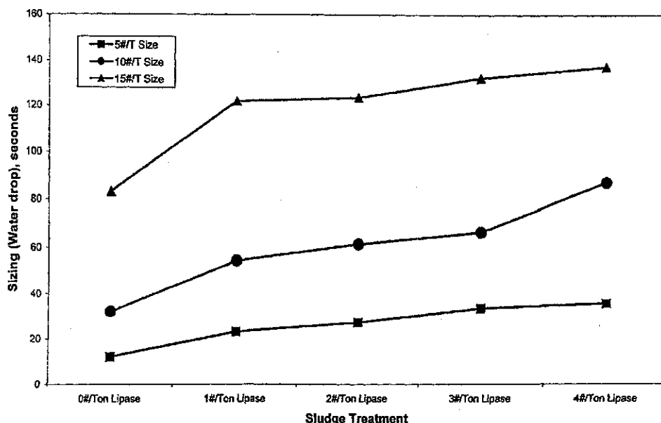
Effect of Lipase Treatment of Sludge on Sizing 10# of Sludge per Ton of Pulp
