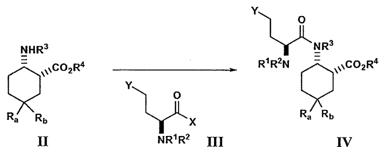
Scheme 1: Preparation of amide IV.
