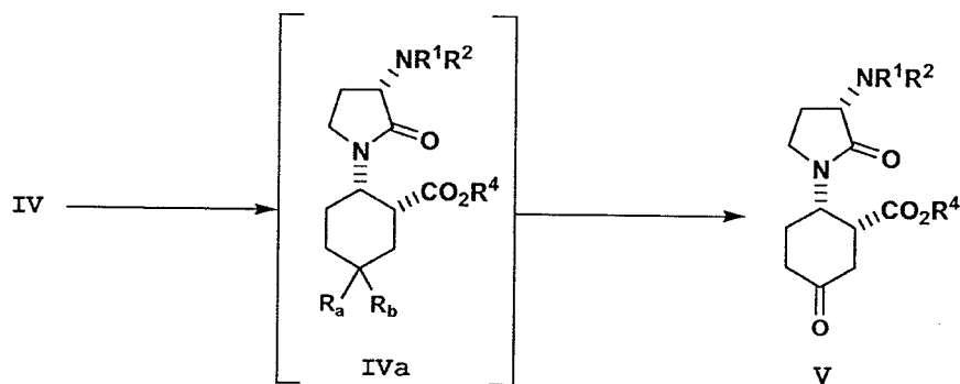
Scheme 2: Preparation of an amide of Formula IV
