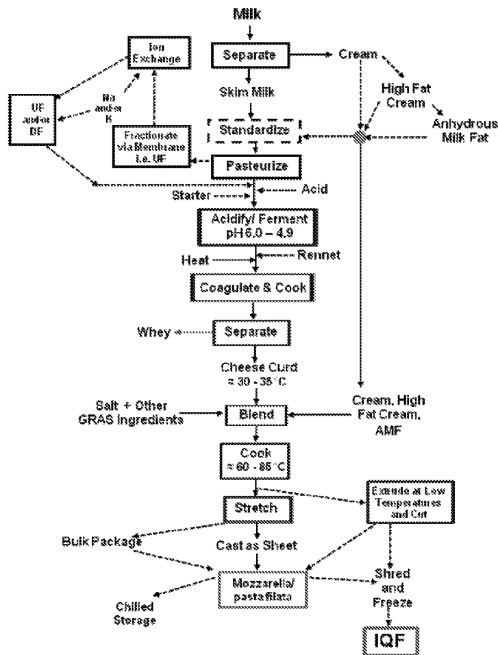
Figure 1: Fonterra Mozzarella manufacturing process
