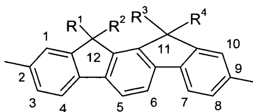
cis-indenofluorene
