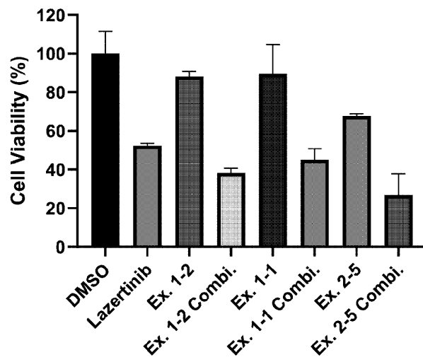
Lazertinib_combination_HCC827
