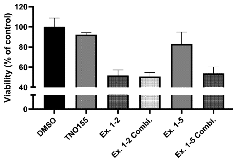
TNO155_Combination_H358
