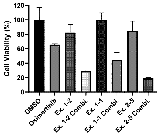
Osimertinib combination_HCC827
