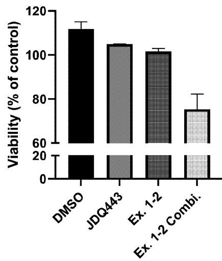
JDQ443_Combination_H358
