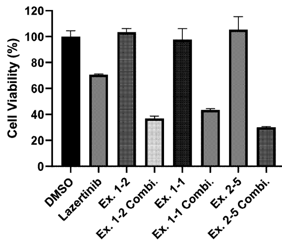
Lazertinib combination_H1975
