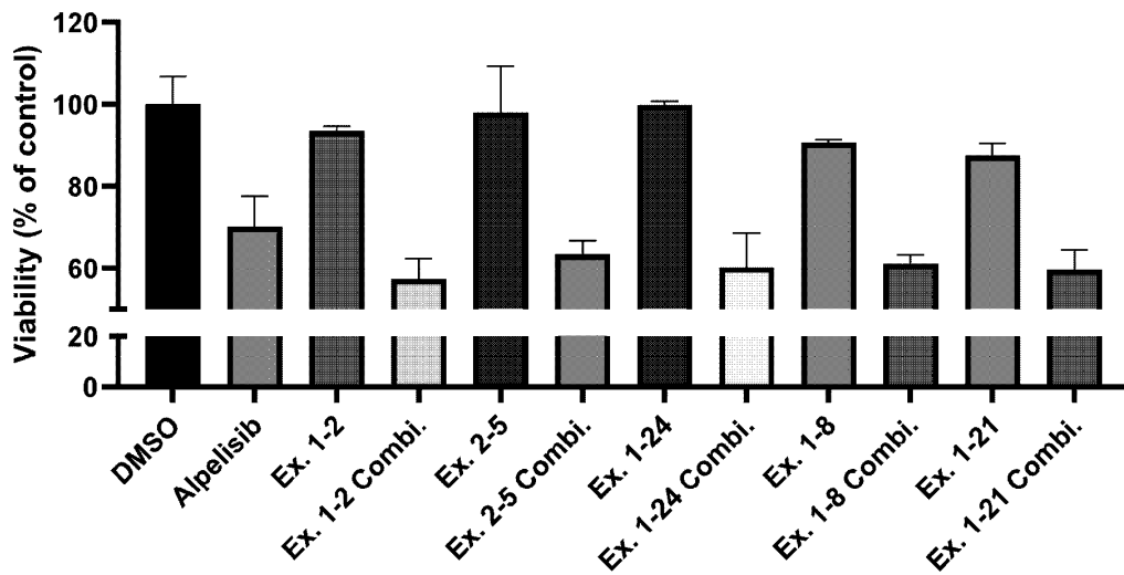
Alpelisib_Combination_MCF7
