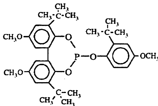
Ligand A
