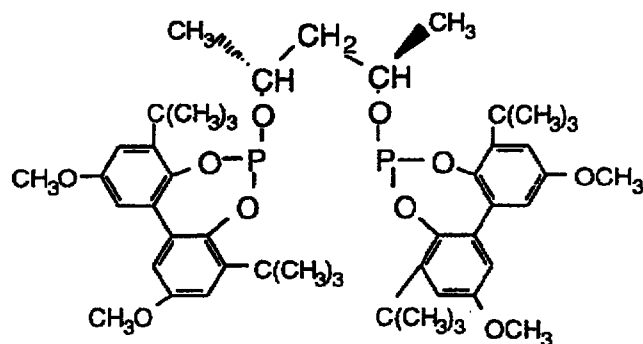
Ligand M
