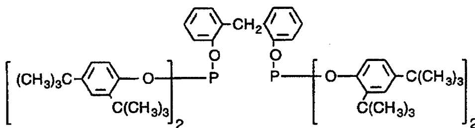
Ligand U
