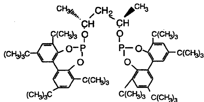
Ligand H
