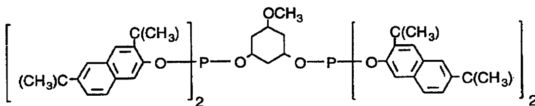
Ligand S
