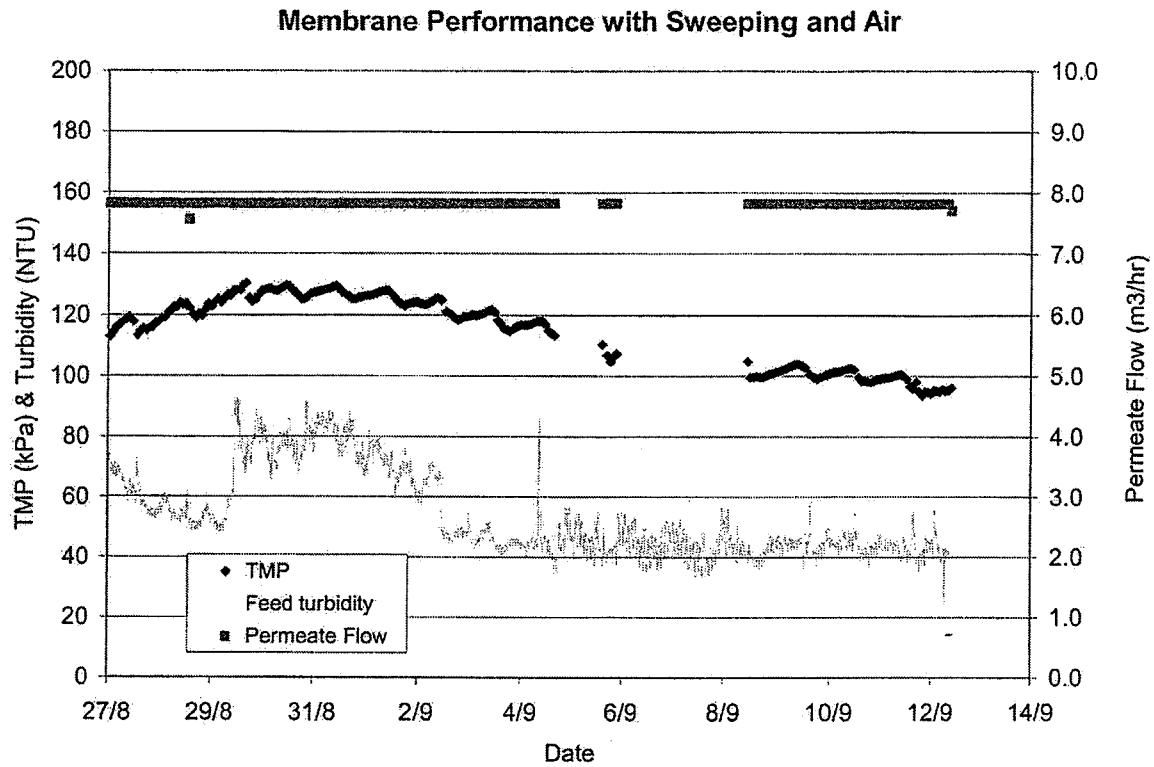
Figure 2 Membrane Filtration Performance with Air Pushed Backwash
