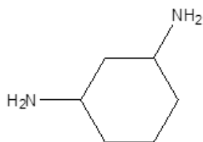
1,3-cyclohexanediamine ,
