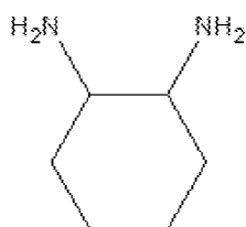
1,2-cyclohexanediamine,
