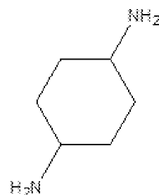
1,4-cyclohexanediamine ,
