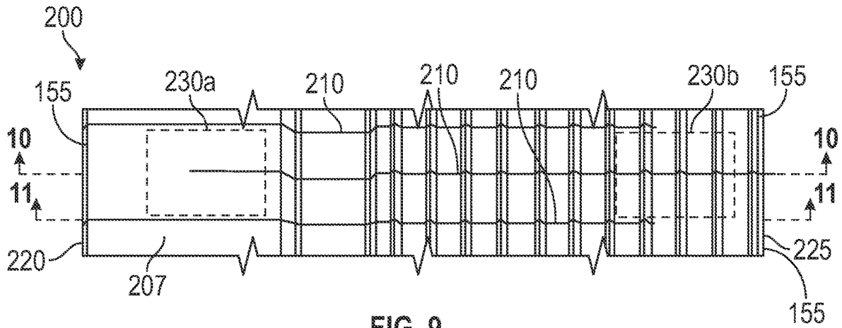
FIG. 9 (Prior Art)
