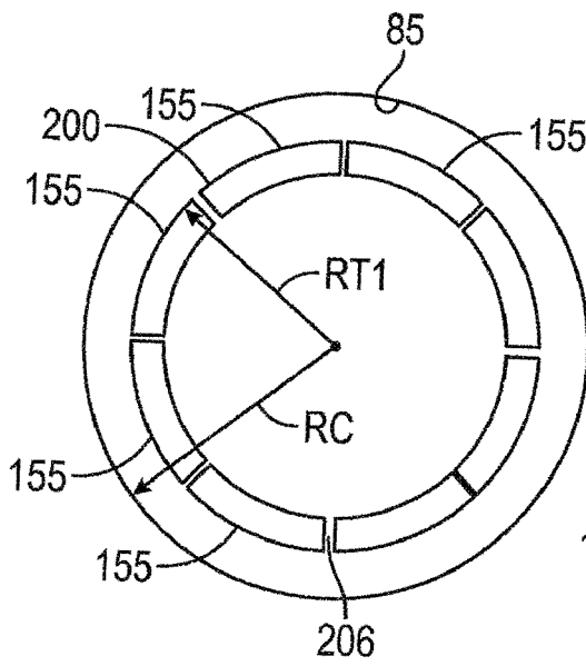
FIG. 5 (Prior Art)
