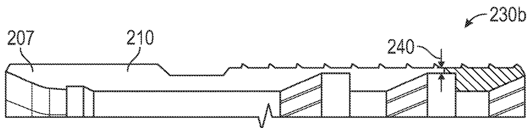
FIG. 11 (Prior Art)
