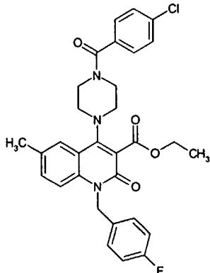
Compound 53
