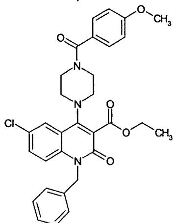
Compound 38 10
