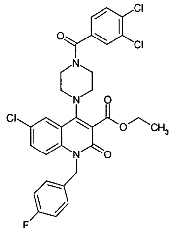
Compound 43
