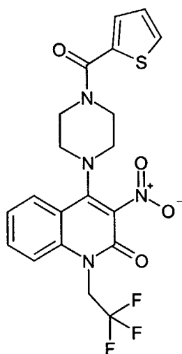
Compound 309
