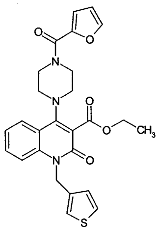
Compound 291
