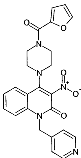
Compound 322
