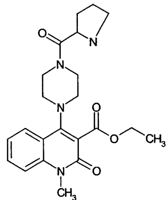
Compound 288
