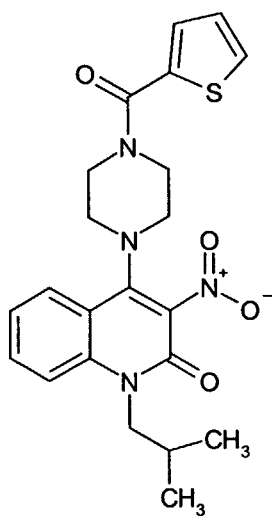
Compound 230
