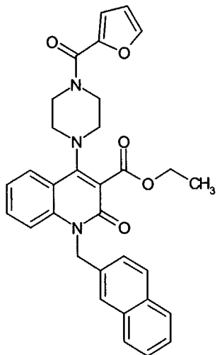
Compound 256
