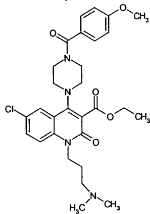
Compound 95
