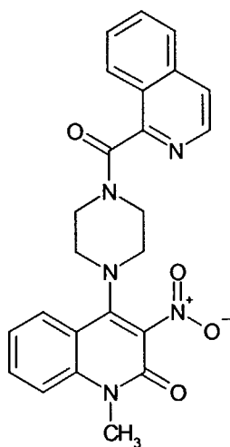
Compound 285
