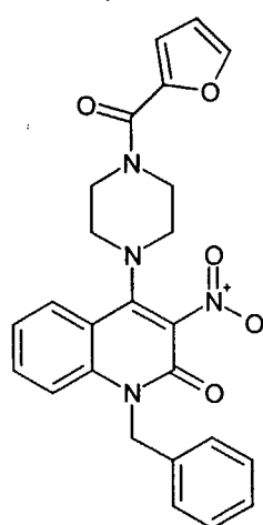
Compound 119
