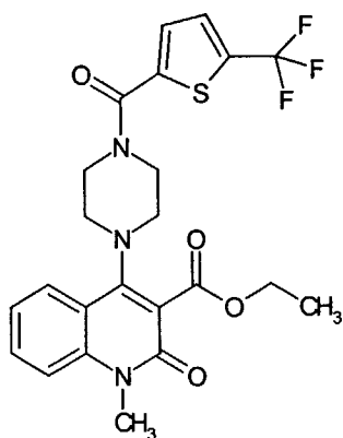
Compound 242
