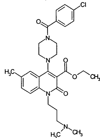
Compound 97
