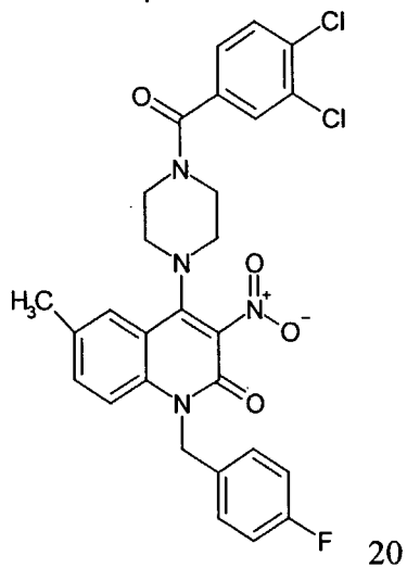
Compound 190
