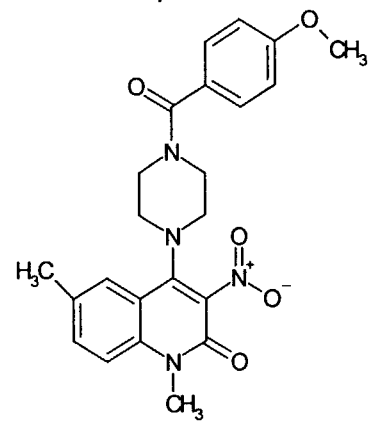
Compound 193
