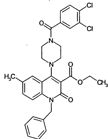
Compound 31
