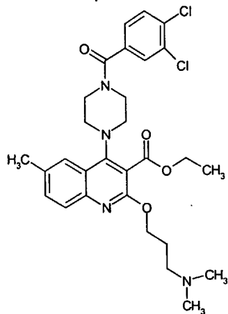
Compound 342
