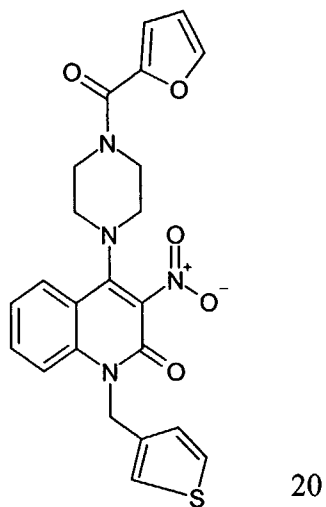
Compound 226
