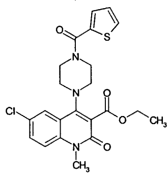
Compound 57
