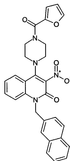
Compound 306
