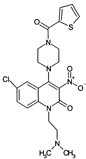
Compound 201
