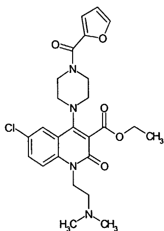
Compound 111
