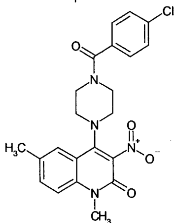
Compound 142
