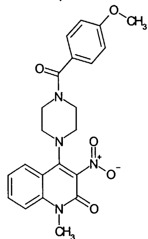
Compound 115
