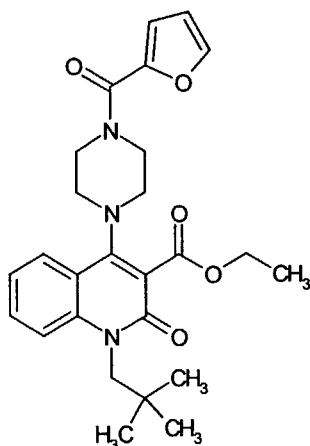
Compound 238
