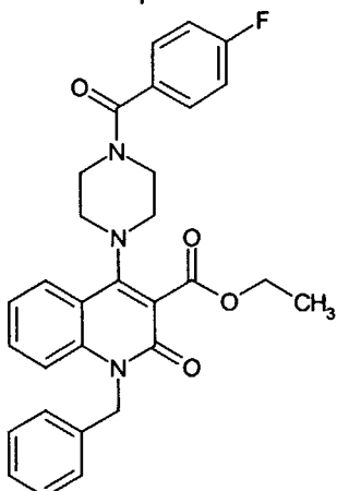
Compound 22
