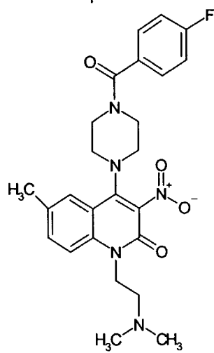
Compound 182
