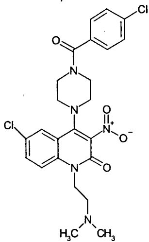
Compound 206
