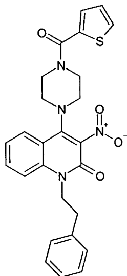
Compound 310
