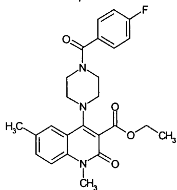
Compound 44
