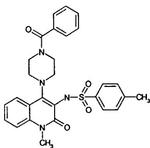
Compound 86
