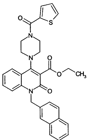
Compound 262
