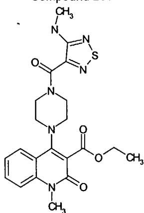
Compound 266
