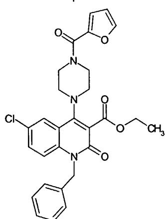
Compound 33
