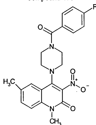
Compound 179
