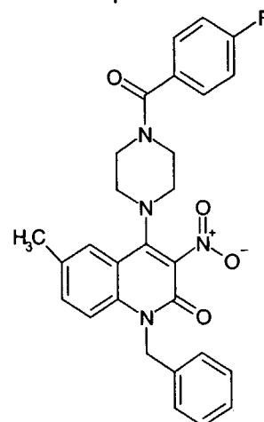
Compound 180
