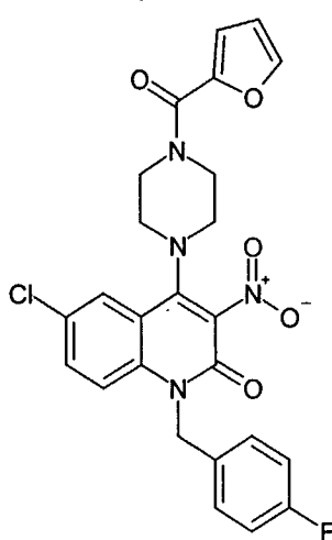
Compound 143
