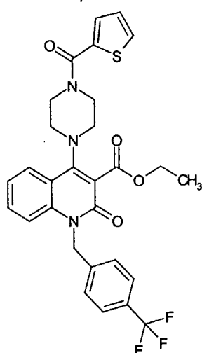
Compound 317
