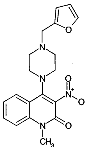
Compound 286
