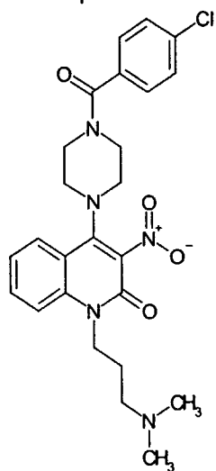
Compound 140
