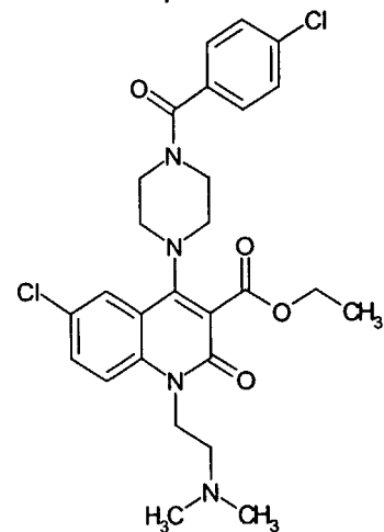
Compound 150
