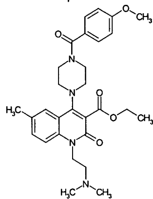
Compound 67
