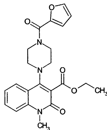
Compound 13
