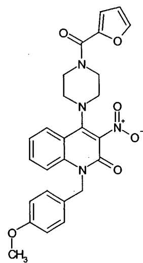
Compound 271
