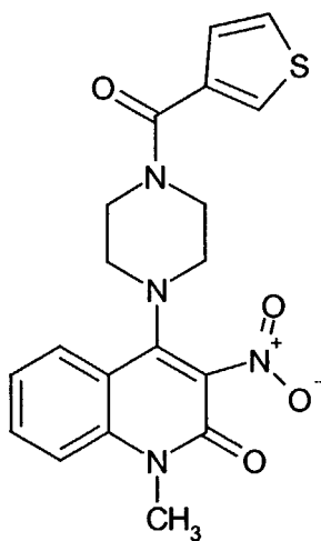
Compound 220
