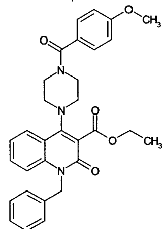
Compound 25
