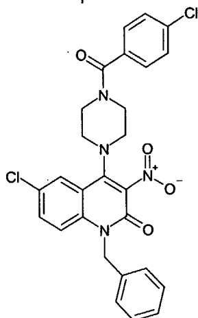
Compound 166
