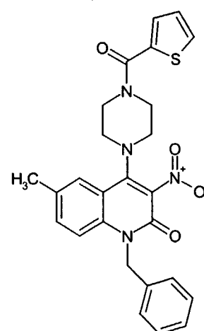
Compound 163
