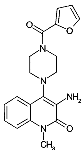
Compound 77
