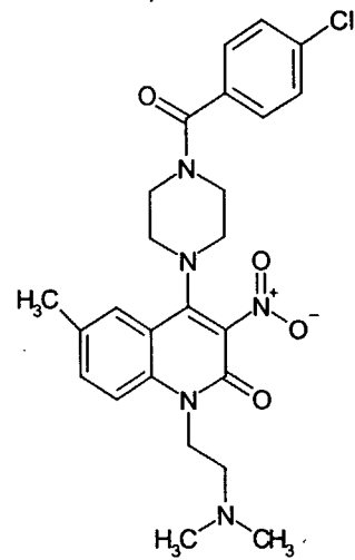
Compound 186
