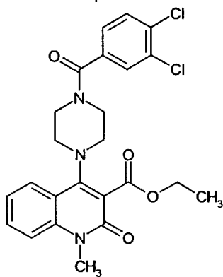
Compound 47
