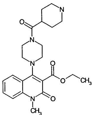
Compound 296
