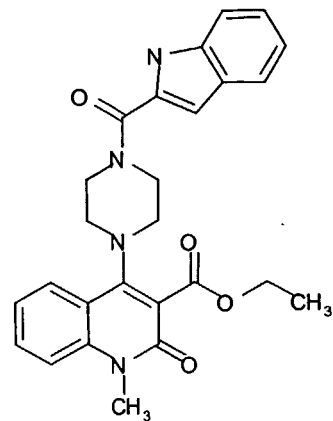
Compound 264
