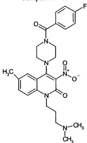
Compound 183
