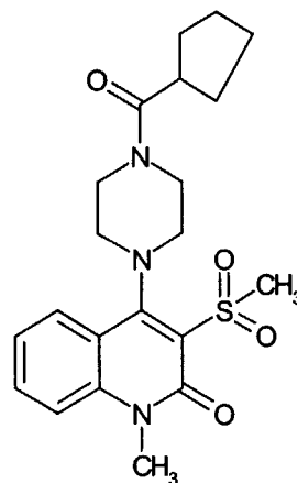
Compound 101
