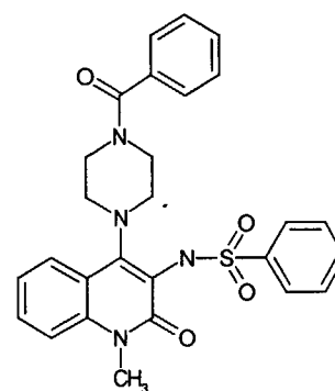
Compound 85
