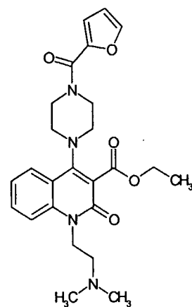
Compound 108
