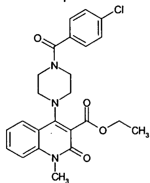
Compound 46
