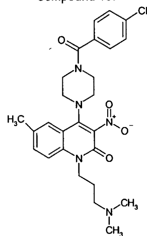
Compound 187
