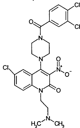
Compound 209
