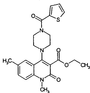
Compound 50
