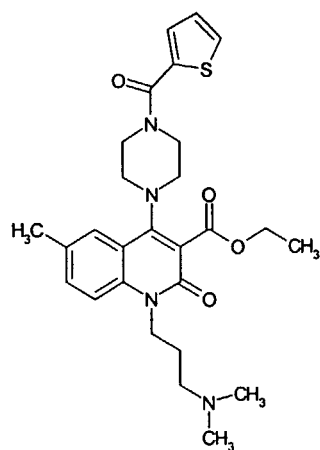
Compound 107
