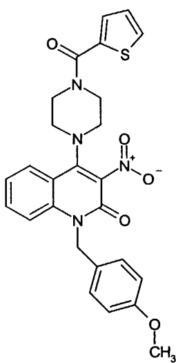
Compound 279
