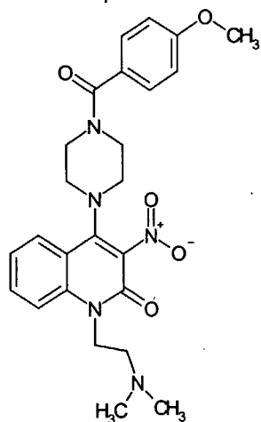
Compound 160
