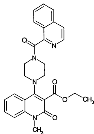
Compound 265
