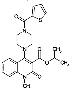
Compound 213
