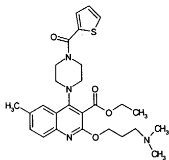
Compound 339
