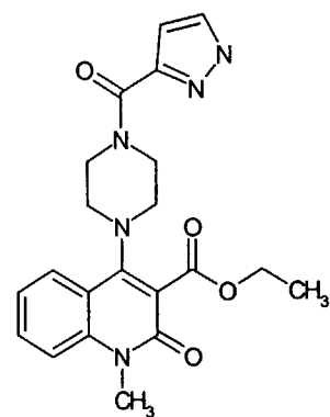
Compound 259
