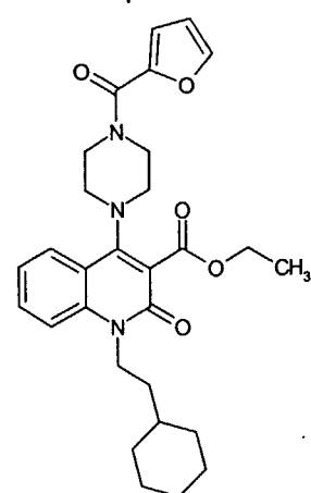
Compound 216
