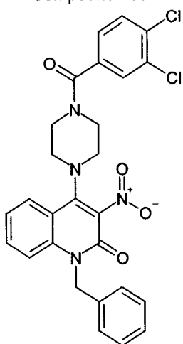
Compound 135
