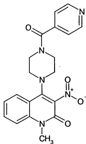
Compound 235
