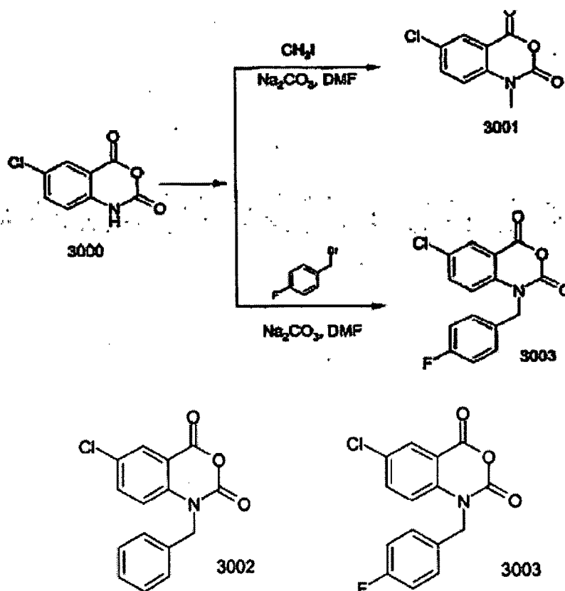
Reaction Scheme 26
