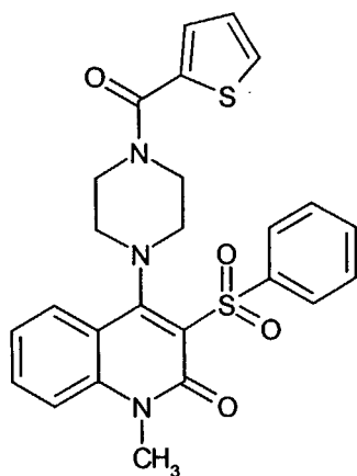
Compound 146
