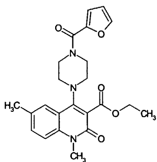
Compound 26
