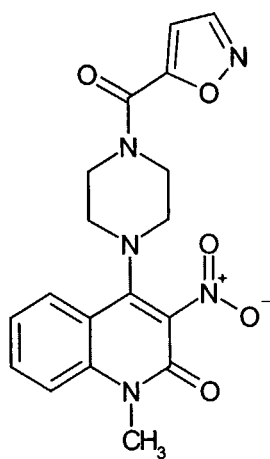
Compound 308
