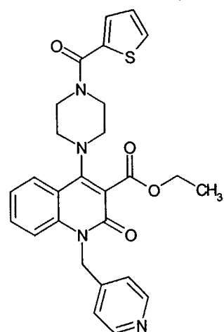
Compound 318
