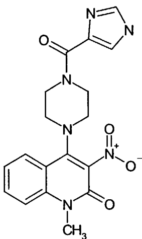
Compound 236
