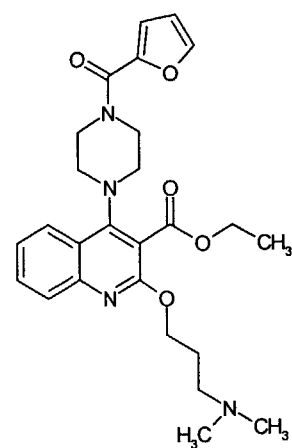
Compound 337
