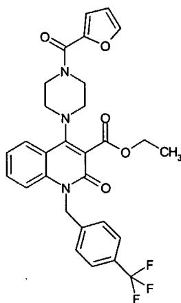
Compound 292
