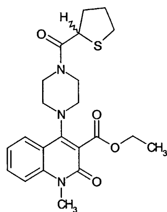
Compound 223
