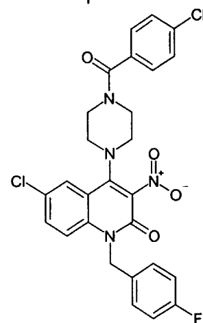
Compound 145
