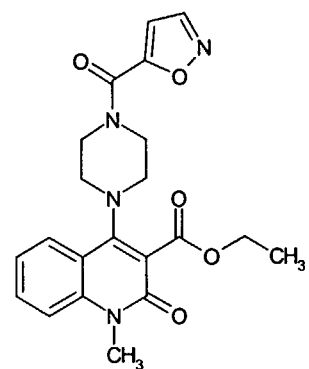
Compound 295
