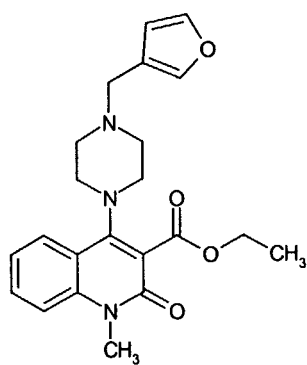
Compound 251
