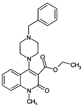
Compound 218
