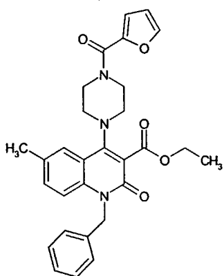
Compound 27
