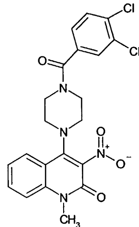
Compound 120
