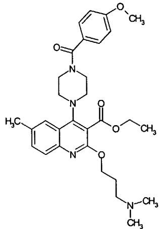
Compound 340
