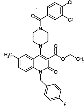
Compound 54
