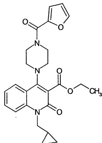
Compound 240
