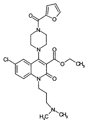
Compound 91
