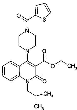
Compound 297
