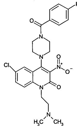
Compound 204
