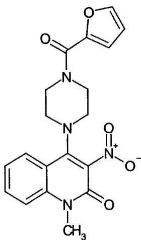
Compound 8
