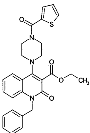
Compound 21
