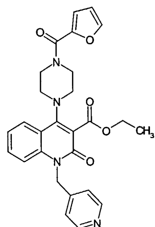
Compound 313
