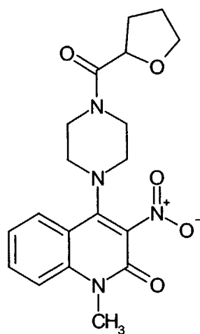
Compound 268
