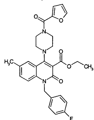
Compound 49
