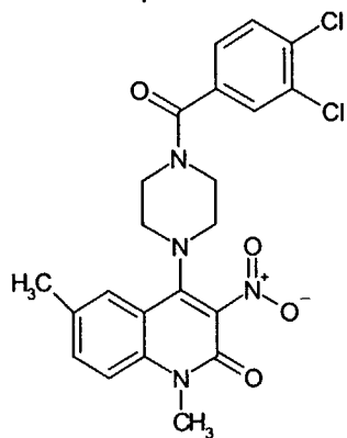
Compound 188 10
