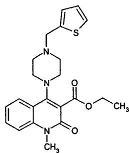
Compound 250
