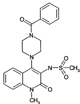
Compound 79
