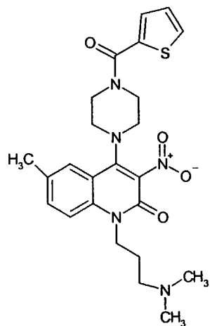
Compound 178
