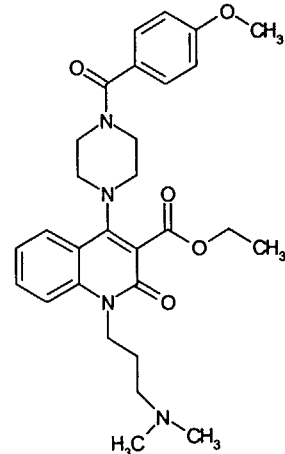
Compound 90
