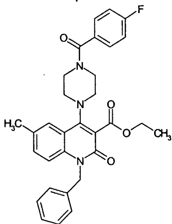
Compound 29
