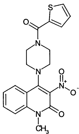
Compound 9
