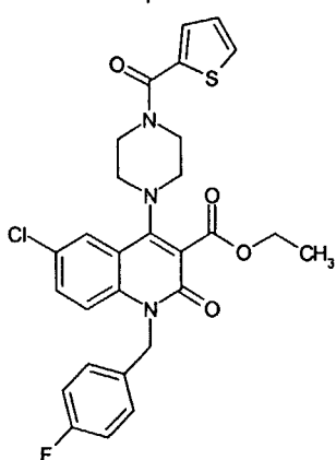
Compound 40
