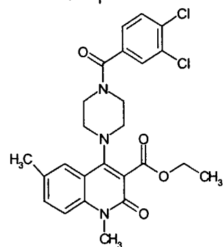
Compound 73
