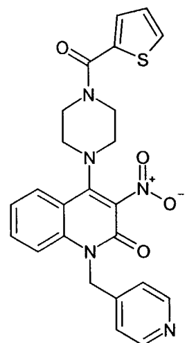
Compound 325
