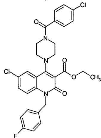
Compound 42
