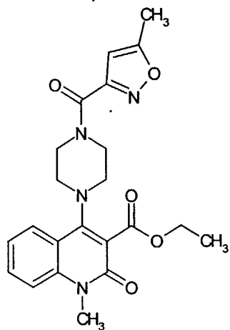
Compound 243
