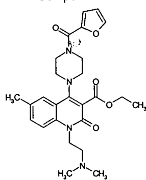
Compound 65
