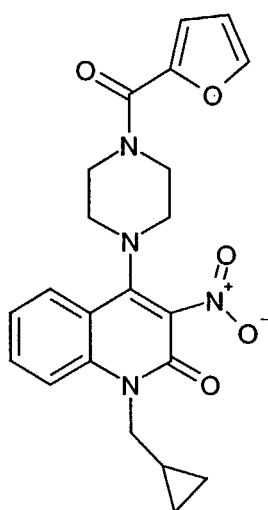
Compound 219
