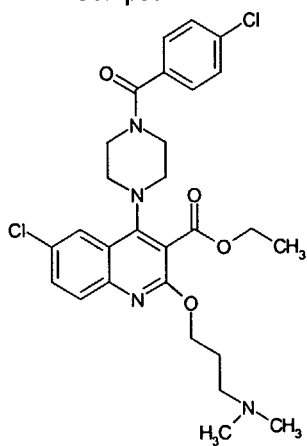
Compound 336
