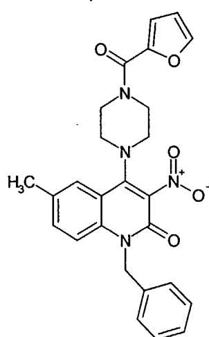
Compound 161
