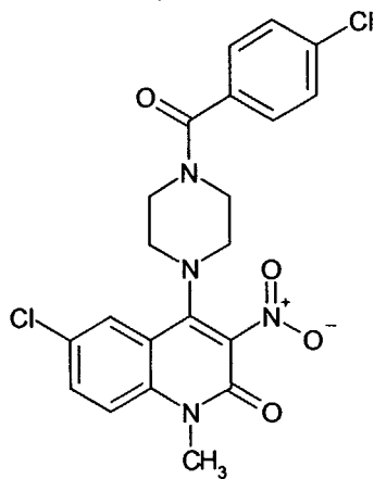
Compound 128 10
