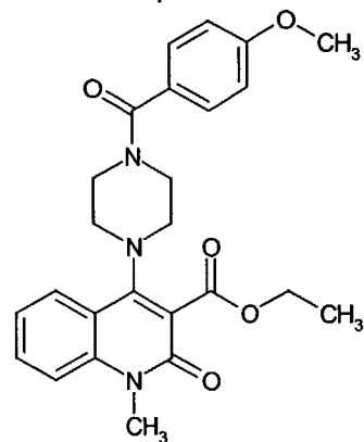
Compound 48
