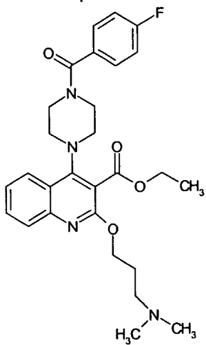
Compound 327
