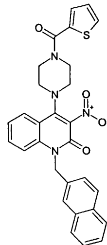
Compound 282
