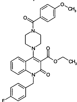
Compound 20
