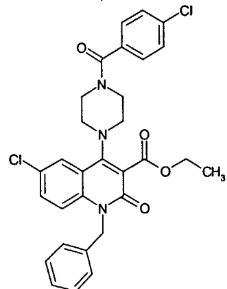
Compound 36
