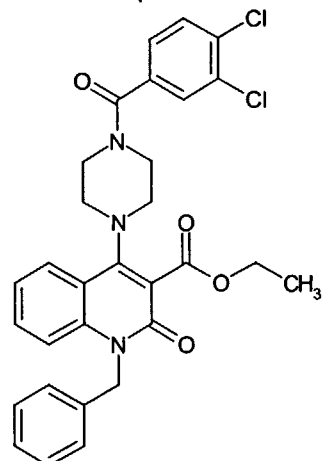
Compound 24
