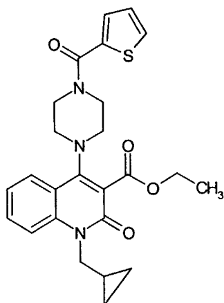
Compound 298
