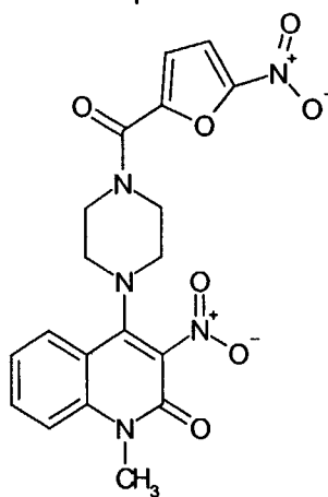
Compound 227
