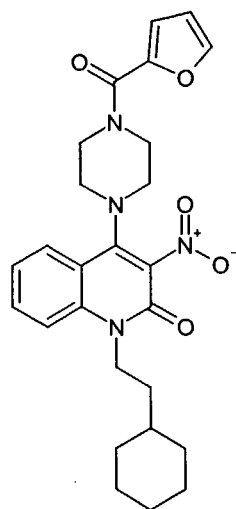
Compound 304
