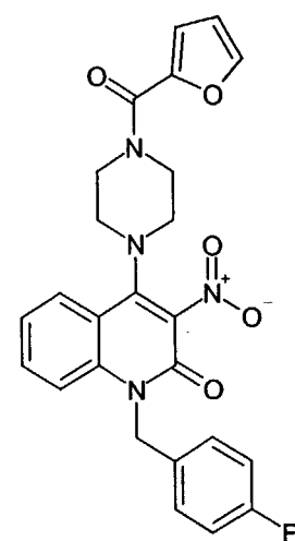
Compound 138
