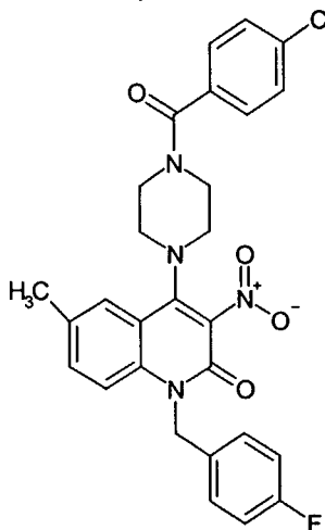
Compound 185
