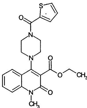
Compound 11
