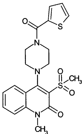
Compound 62
