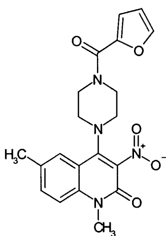
Compound 173
