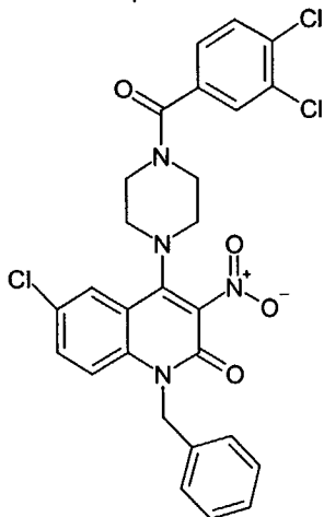
Compound 208
