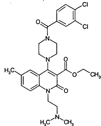
Compound 168
