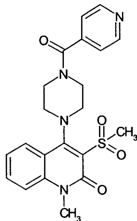
Compound 100
