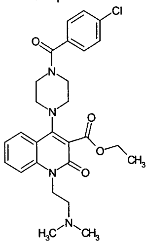
Compound 153
