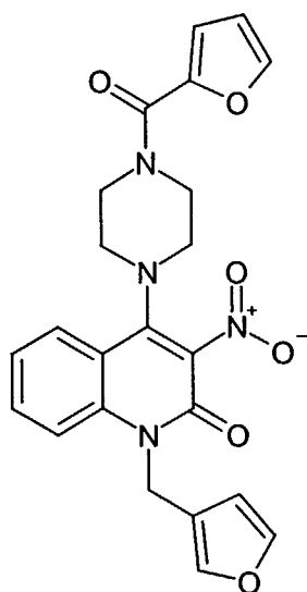
Compound 321
