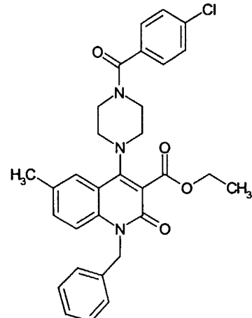
Compound 30
