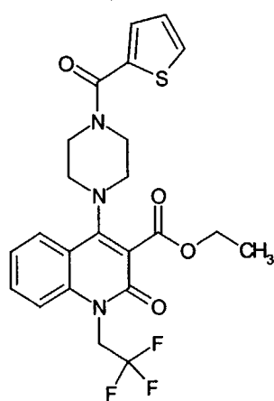
Compound 245
