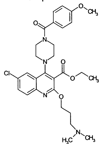
Compound 332
