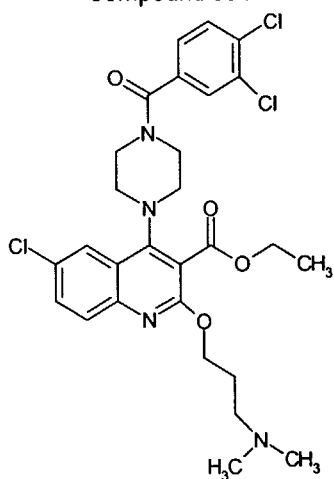
Compound 334
