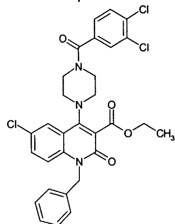
Compound 37
