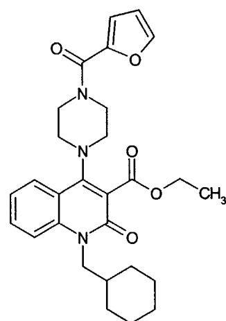
Compound 241
