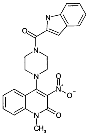
Compound 284
