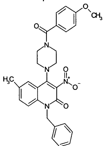
Compound 194
