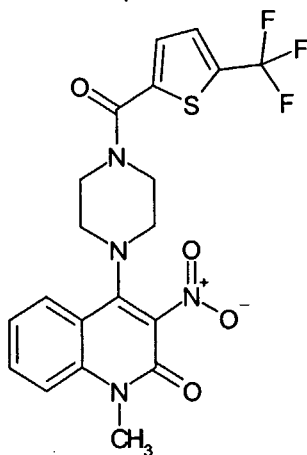
Compound 274
