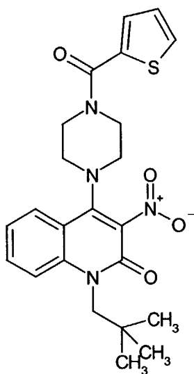
Compound 254
