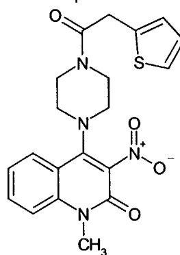
Compound 215
