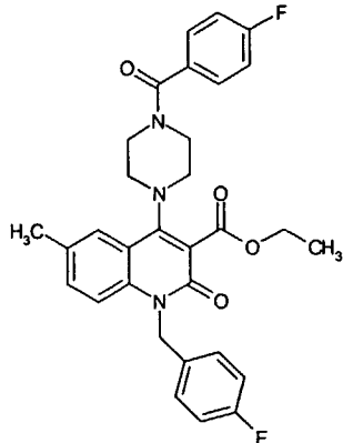
Compound 52
