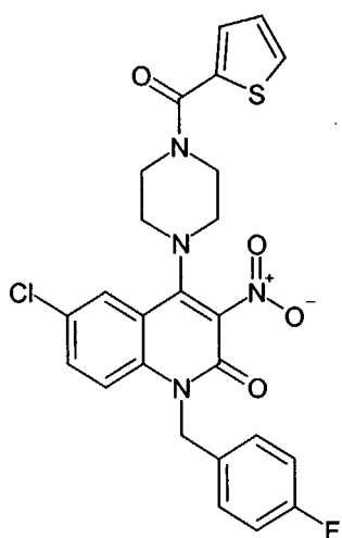
Compound 147
