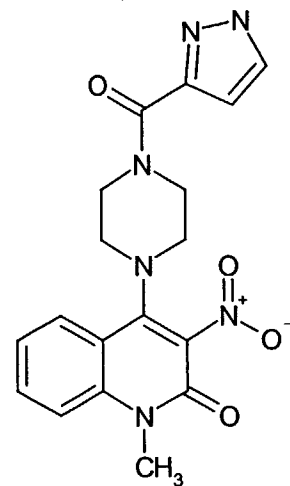
Compound 228
