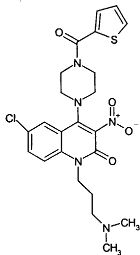
Compound 202
