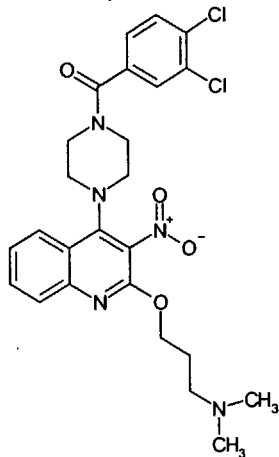
Compound 341
