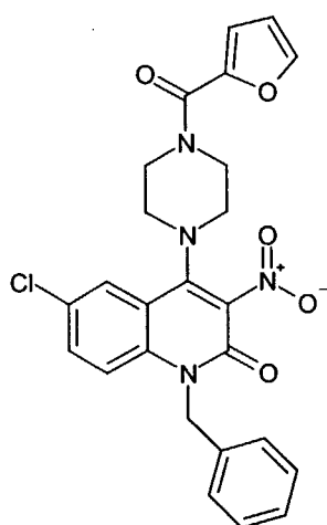
Compound 165
