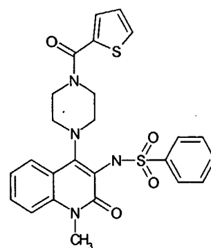
Compound 84
