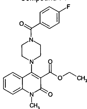
Compound 71
