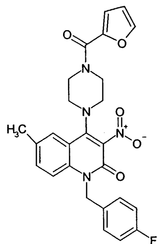
Compound 174
