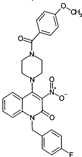
Compound 116
