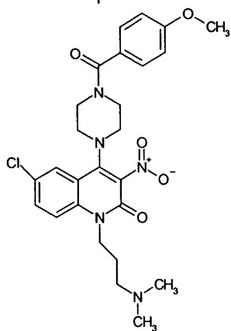
Compound 212
