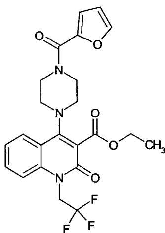
Compound 239
