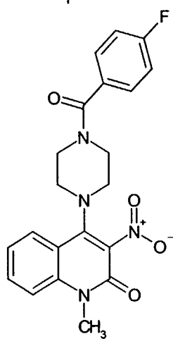
Compound 123
