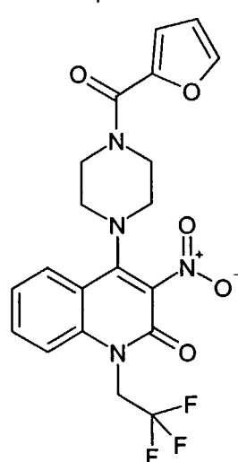
Compound 253
