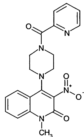
Compound 234
