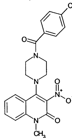
Compound 121
