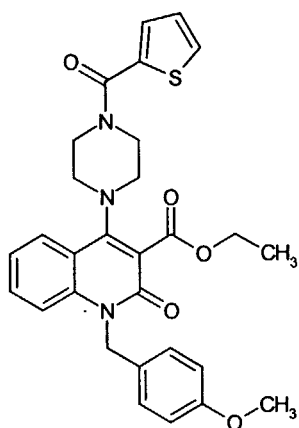
Compound 261
