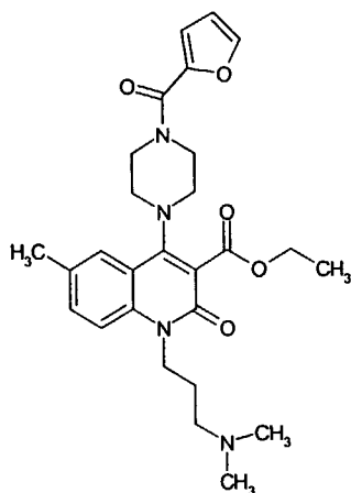
Compound 112
