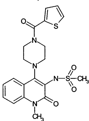
Compound 45
