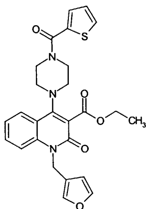
Compound 315
