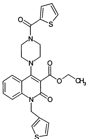
Compound 224
