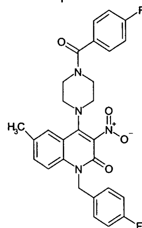
Compound 181
