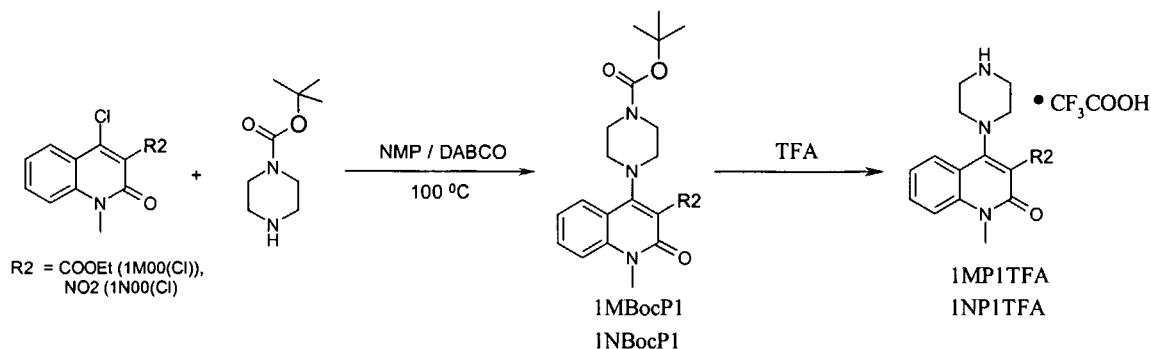
Reaction Scheme 15
