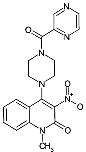
Compound 311
