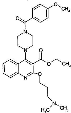
Compound 329
