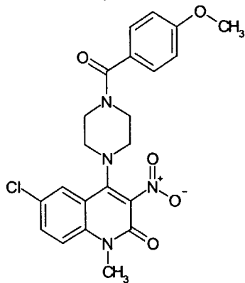
Compound 130
