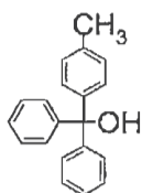
(Compound 24)
