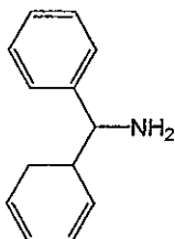
Aminodiphenylmethane
