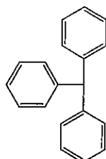
Triphenylmethane
