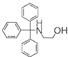
2-(Triphenylmethylanino)ethanol (Compound 3)
