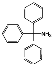
Triphenylmethanamine
