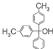
(Compound 23)
