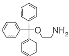
2-(Triphenylmethyloxy)ethylamine (Compound 4)
