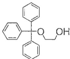
2-(Triphenylmethyloxy)ethanol (Compound 2)
