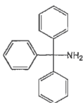
Triphenylmethanamine
