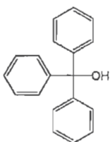
Triphenylmethanol
