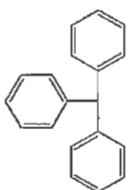
Triphenylmethane
