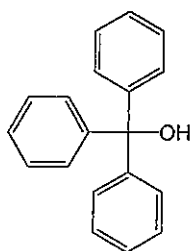
Triphenylmethanol
