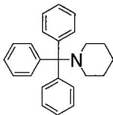
1-(Triphenylmethyl)piperidine (Compound 5)
