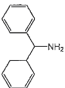
Aminodiphenylmethane
