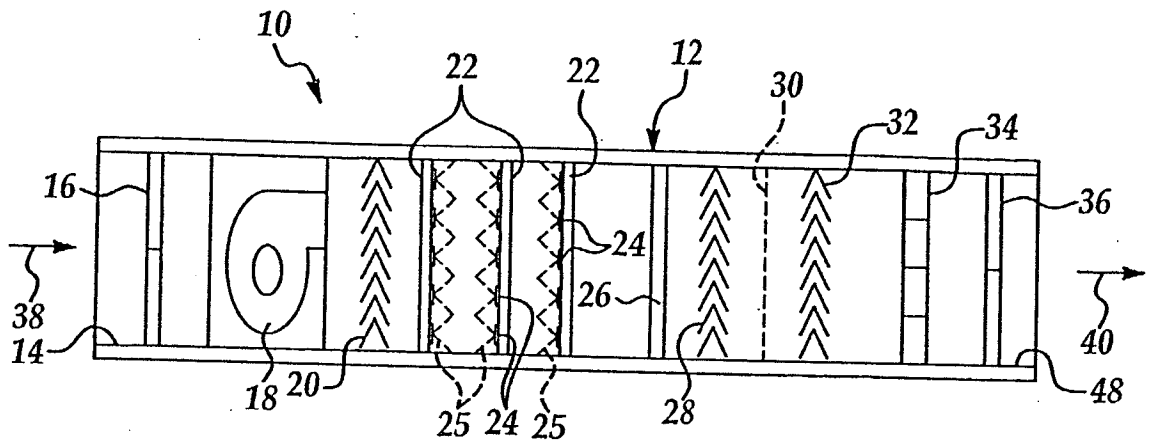
Figure 1 Prior Art
