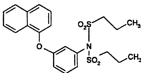
3-(Naphthyl-1-oxy)-1-bis-N-(1-propylsulfonyl)aminobenzene (Example 3)
