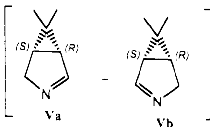
Racemic Mixture
