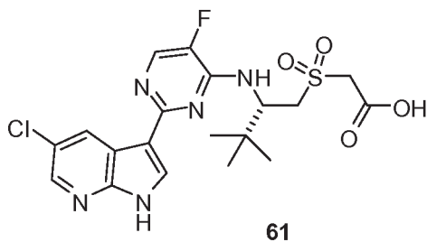
( S )-2-(2-(2-(5-chloro-1 H -pyrrolo[2,3- b ]pyridin-3-yl)-5-fluoropyrimidin-4-ylamino)-3,3-dimethylbutylsulfonyl)ethanoic acid ( 61 )
