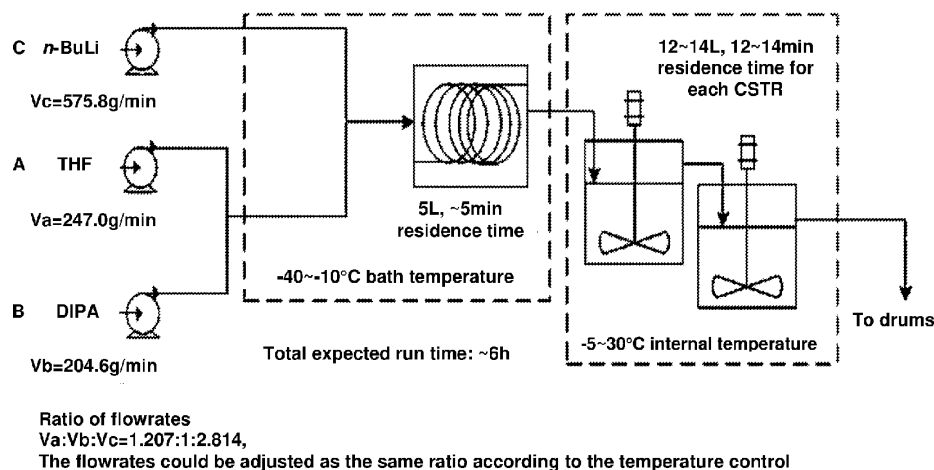
Process flow diagram (PFD) for LDA preparation
