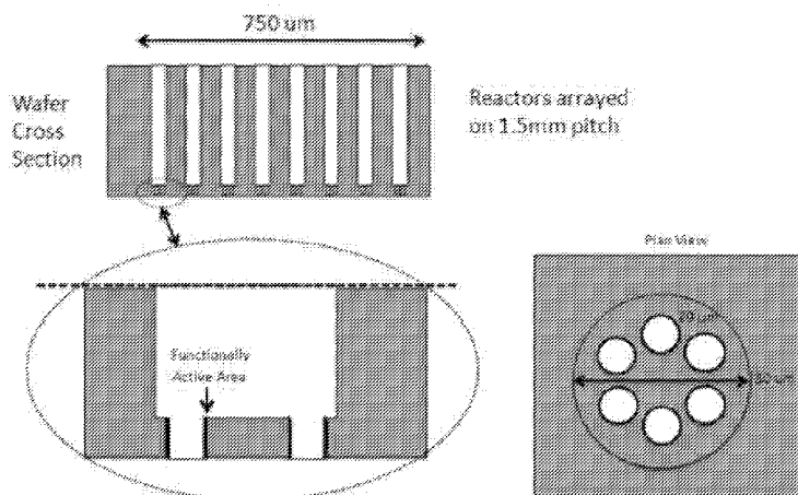
Figure 4 Oligo Wafer Reactor
