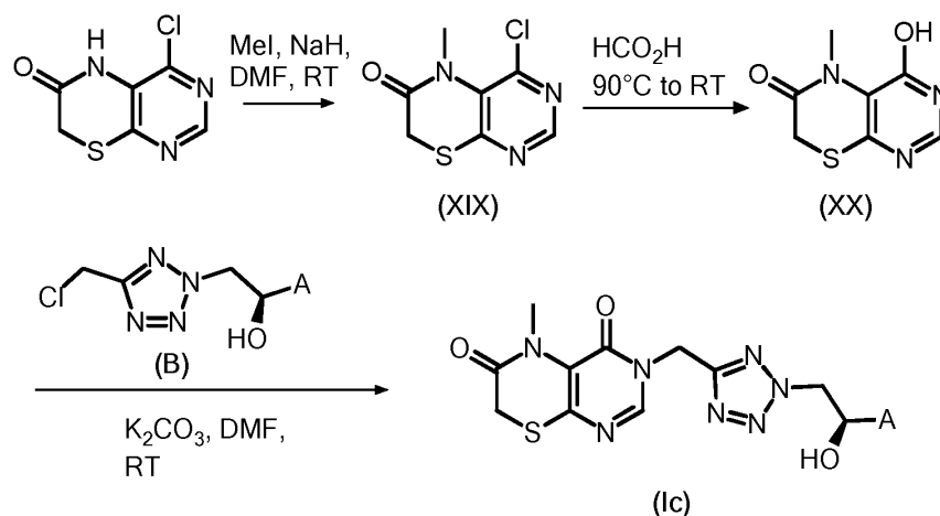
10 Scheme 5:
