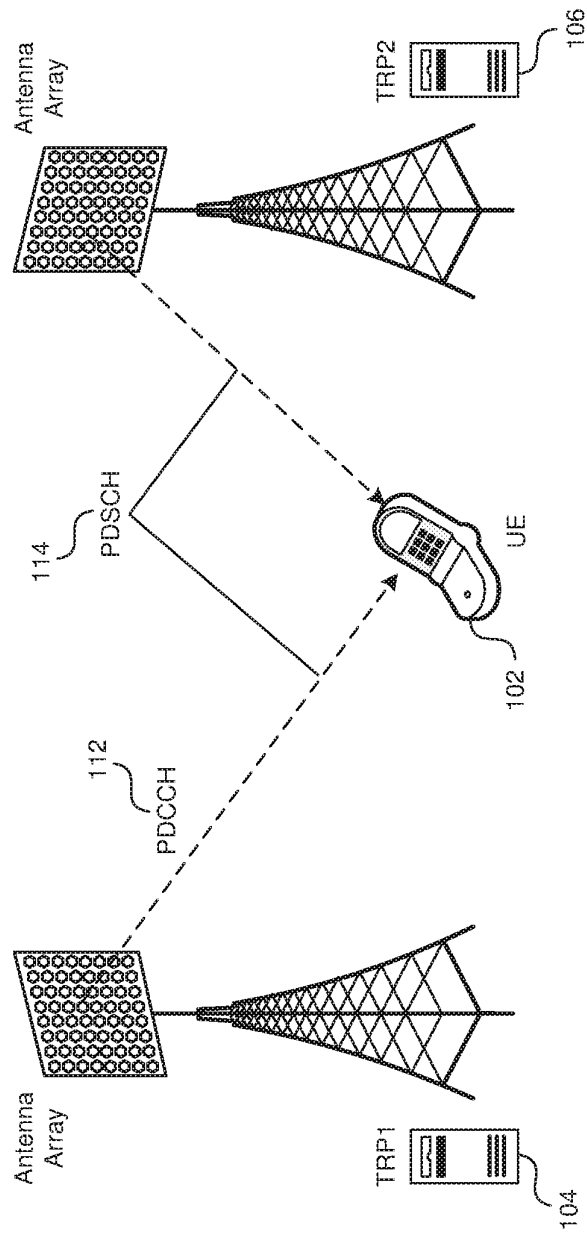
Scheme 2: Single PDCCH/PDSCH
