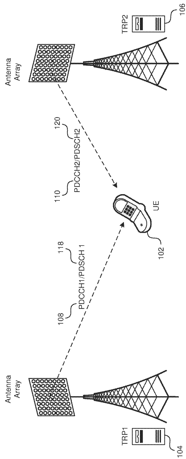
Scheme 1: Multiple PDCCH/PDSCH
