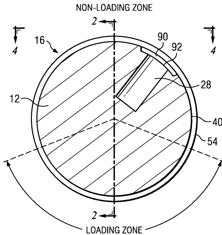
FIG. 3 (PRIOR ART)
