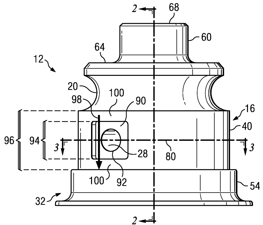
FIG. 4 (PRIOR ART)
