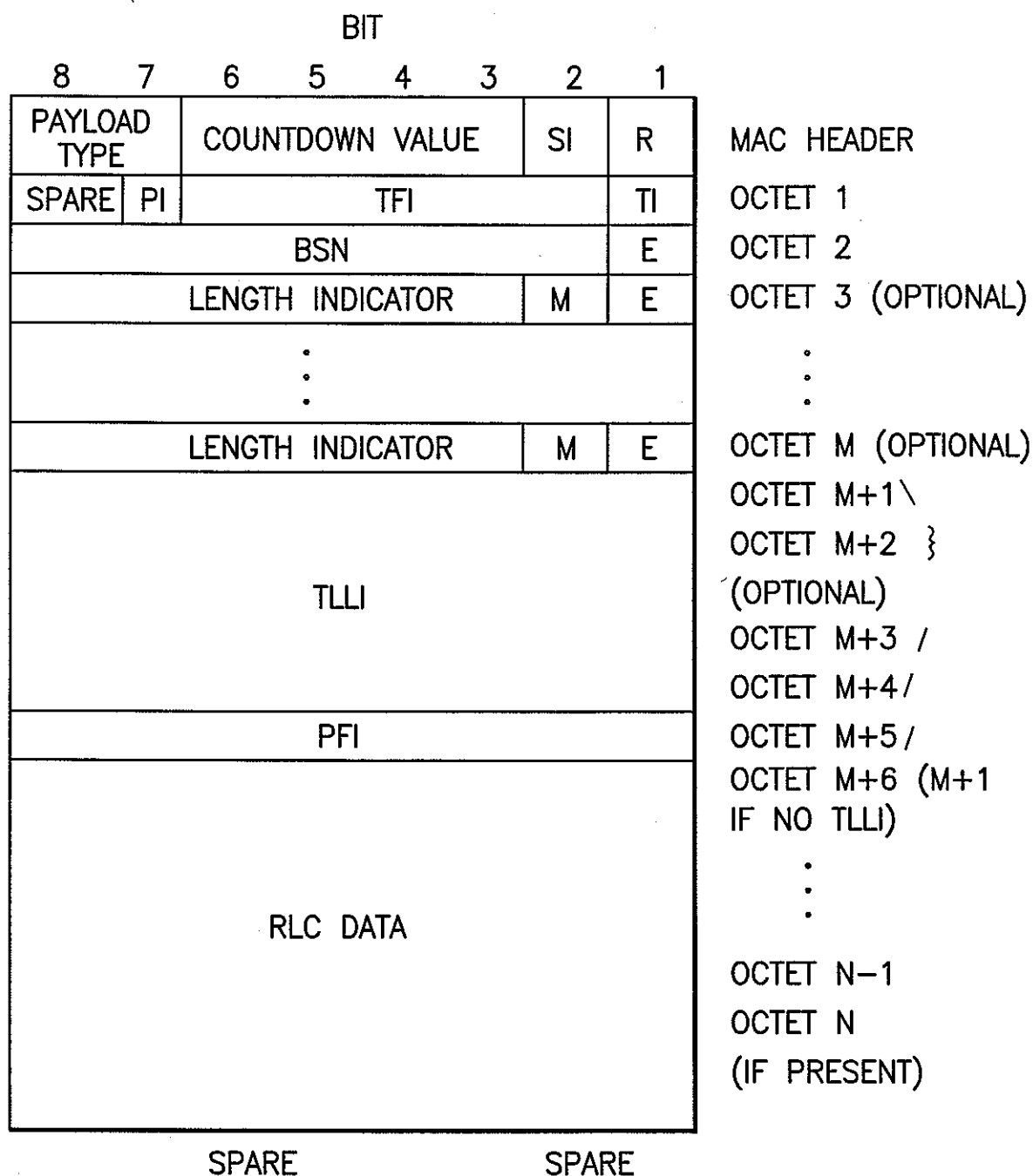
GPRS UPLINK RLC DATA BLOCK WITH MAC HEADER
