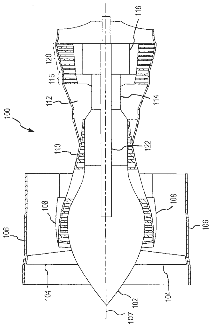
FIG.1 PRIOR ART
