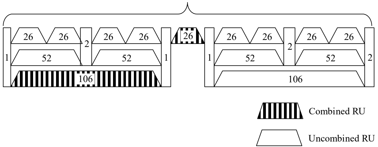
RU distribution in a 20 MHz frequency band range in 80 MHz
