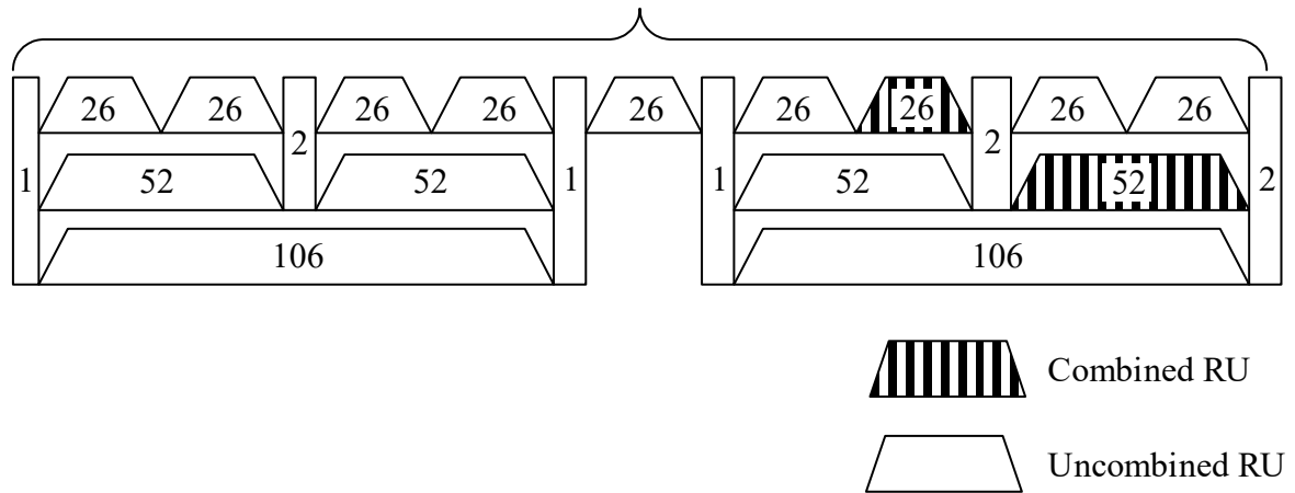
RU distribution in first 20 MHz or second 20 MHz in 80 MHz
