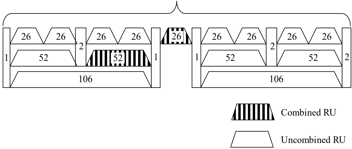
RU distribution in a 20 MHz frequency band range in 80 MHz
