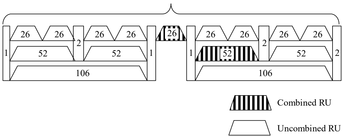
RU distribution in a 20 MHz frequency band range in 80 MHz
