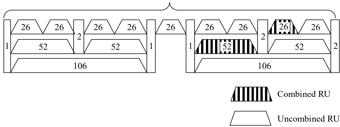
RU distribution in a third 20 MHz frequency band range or a fourth 20 MHz frequency band range in 80 MHz
