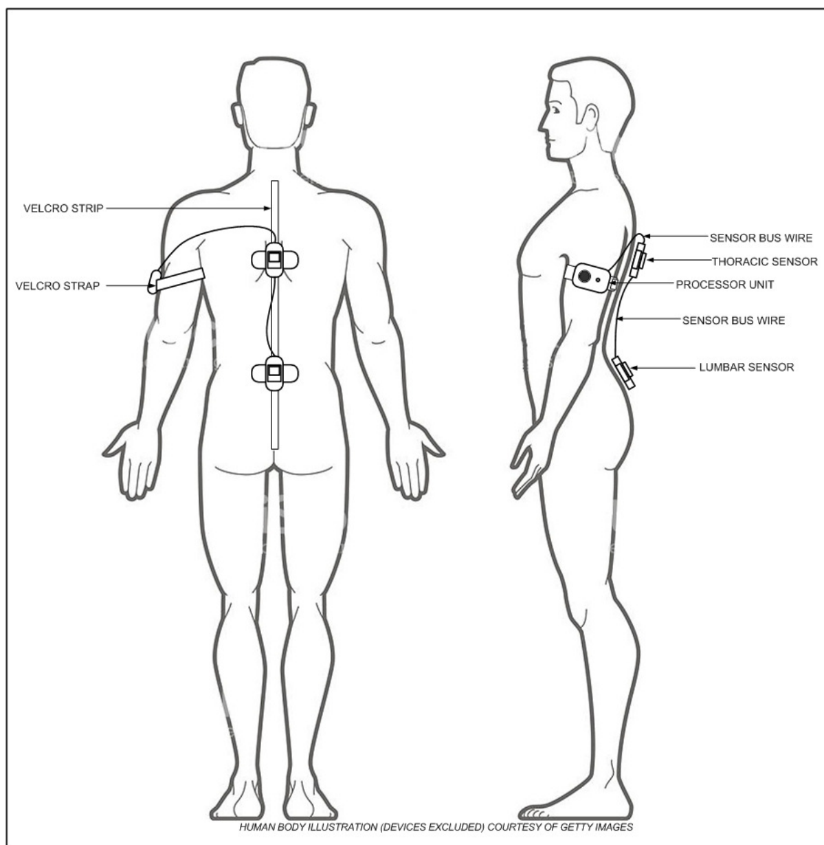
Figure 1. Full Assembly of Apparatus
