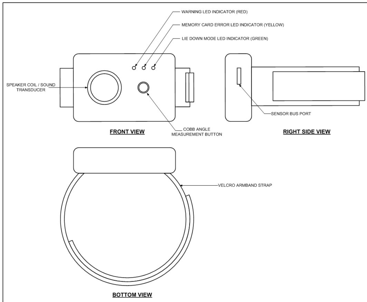
Figure 2. Main Processor Unit Illustration
