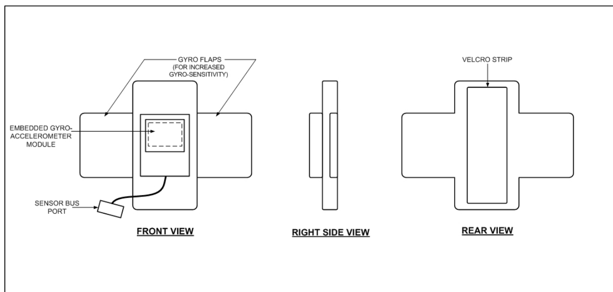
Figure 3. Thoracic and Lumbar Sensor
