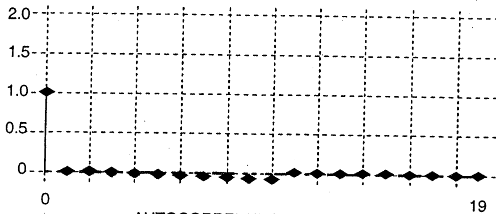
AUTOCORRELATION ANALYSIS
