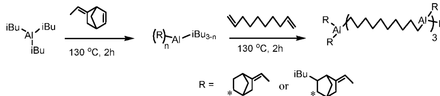
Reaction Scheme 2.
