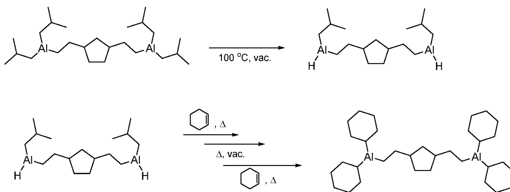
Reaction Scheme 11.
