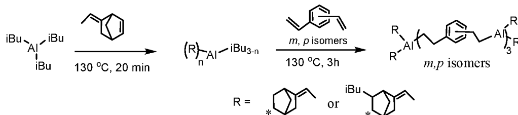
Reaction Scheme 3.
