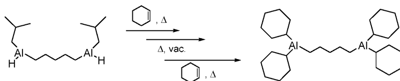
Reaction Scheme 6.
