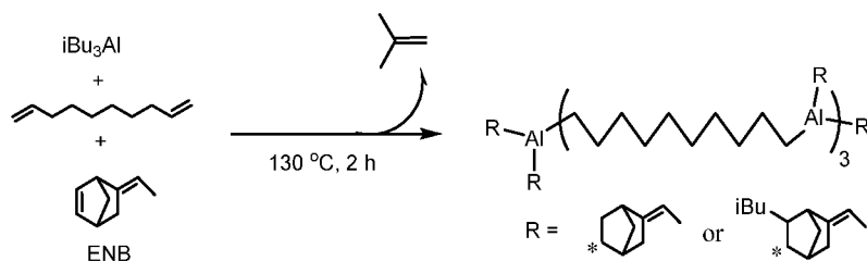
Reaction Scheme 1.
