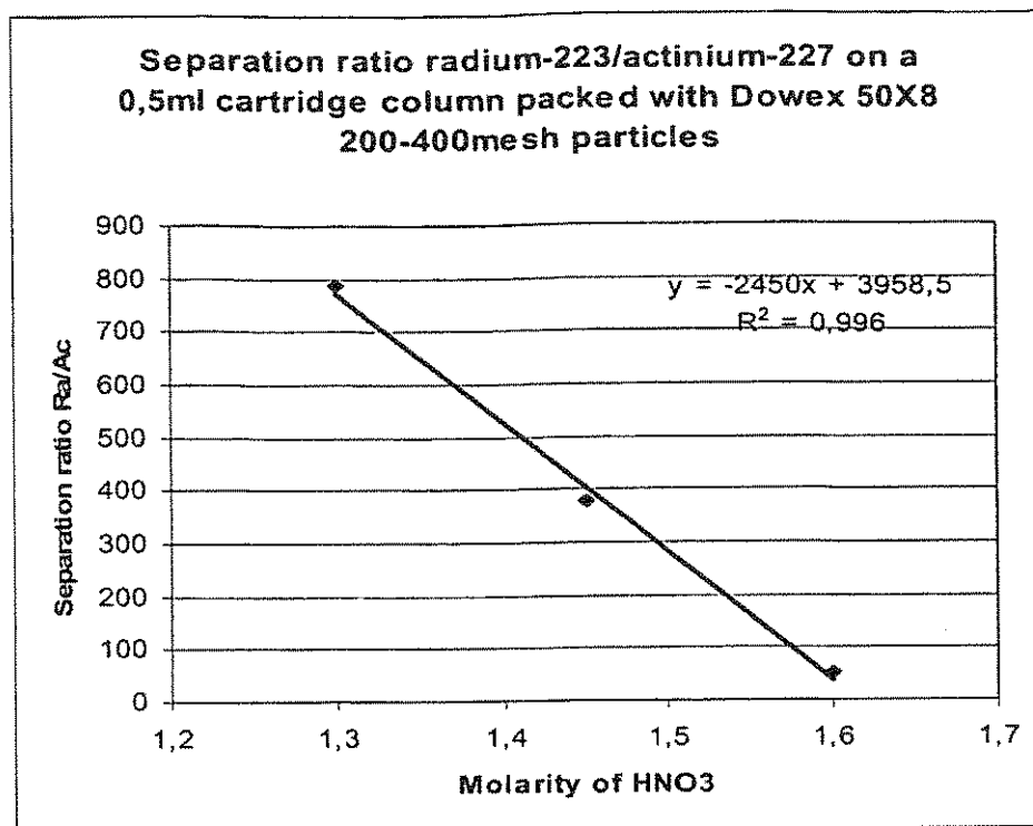
Figure 7 separation ratio between radium-223 and actinium-227 at varying HNO 3 concentrations.
