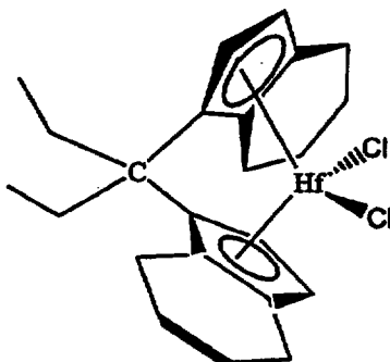
methylphenylsilylbis( \eta^5 -4,5,6,7-tetrahydro-1-indenyl)zirconium dichloride;
