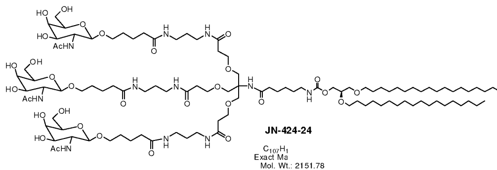
Formula II
