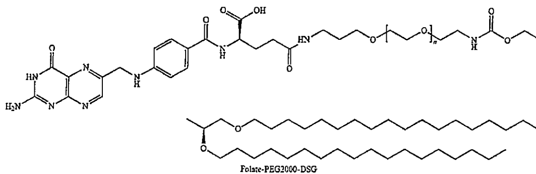
Formula VII
