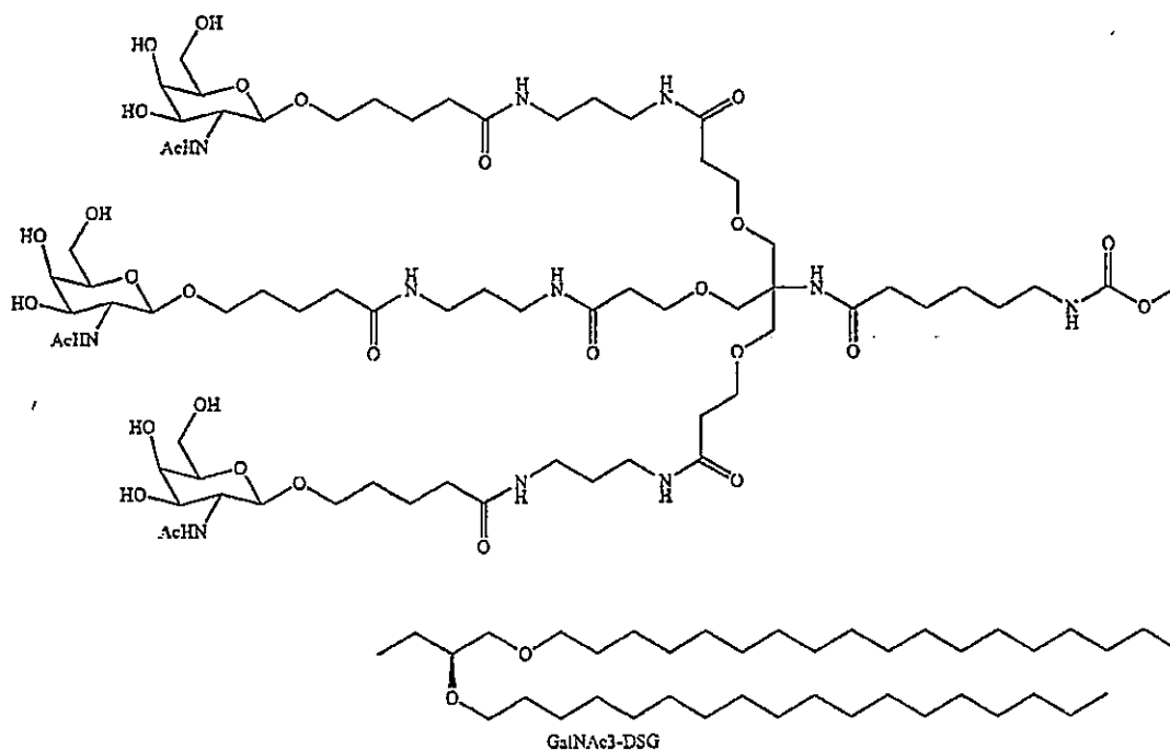
Formula II
