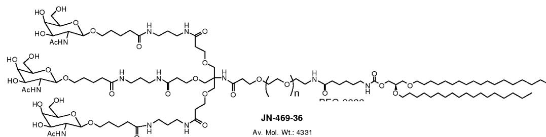
Formula III
