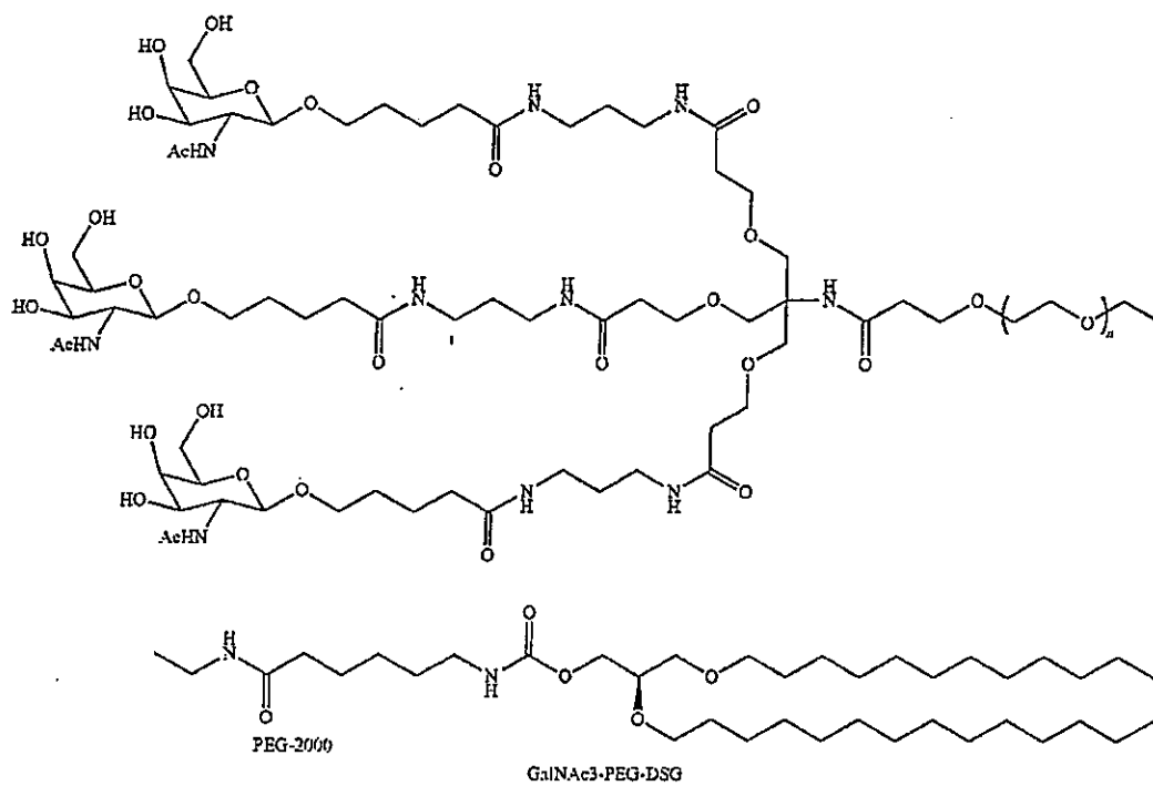
Formula III
