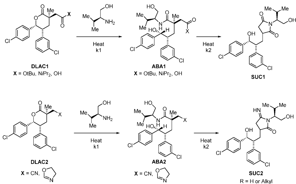
[0112] Scheme 2. Attempted Preparation of Analogues of ABA ( k_1 \approx k_2 )
