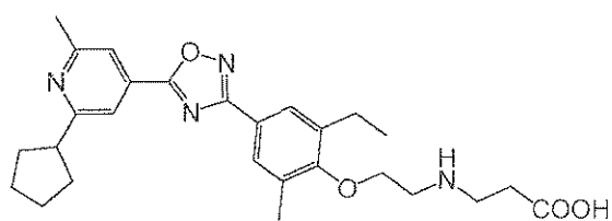
Compound 1, close analog of Example 1 within scope of D1
