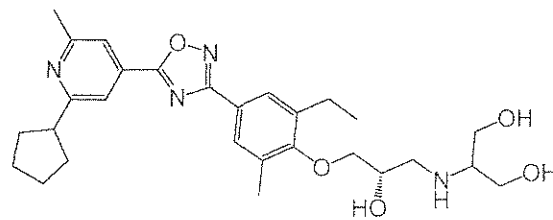
Compound 4, close analog of Example 4 within scope of D1
