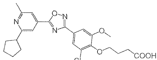
Compound 8, close analog of Example 35
