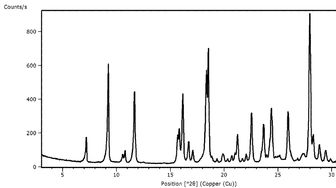
FIG. 2. Form 3 XRPD
