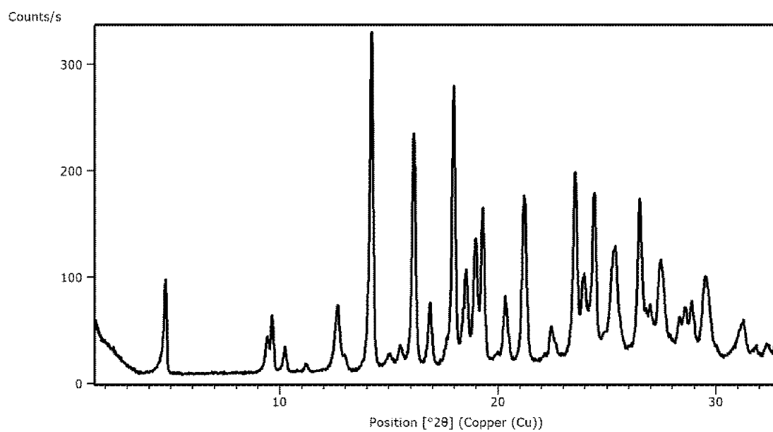
FIG. 4. Form 8 XRD
