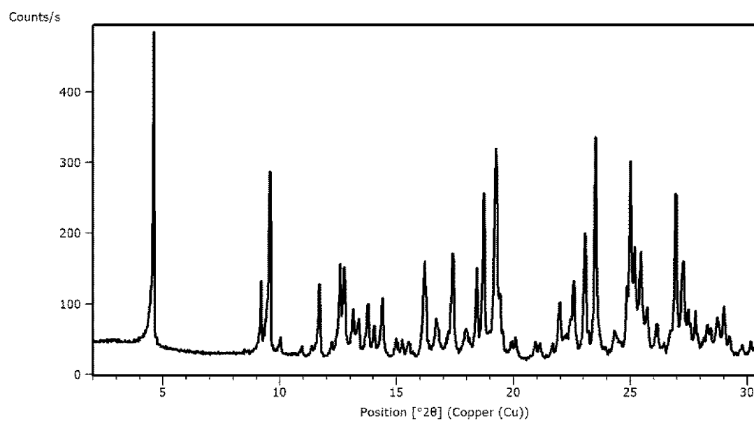
FIG. 1. Form 1 XRPD
