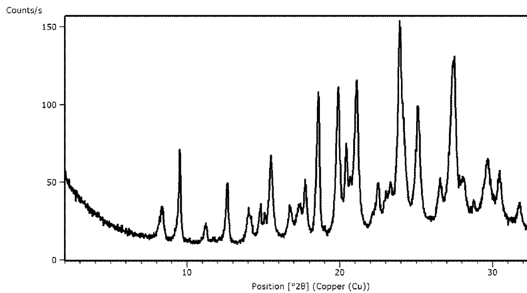
FIG. 3. Form 5 XRPD
