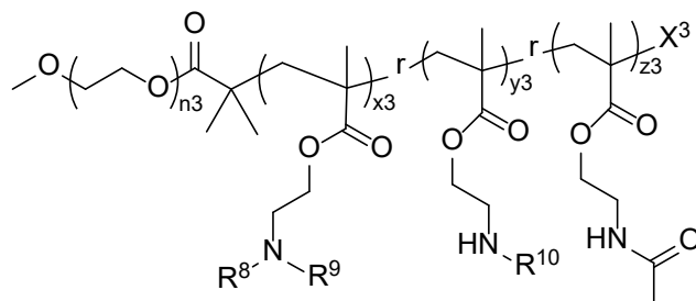
Formula (III),
