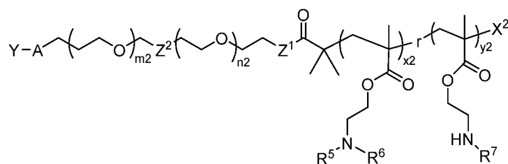
Formula (II-a),
