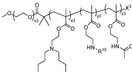
Formula (IV),
