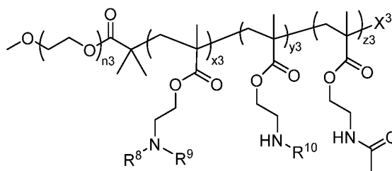
Formula (III-c).
