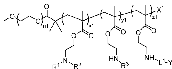
Formula (I-c).
