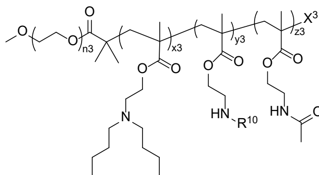
Formula (IV),
