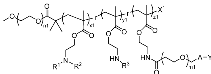
Formula (I-a),
