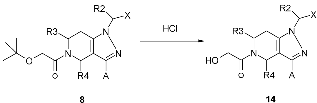
15 Scheme 11
