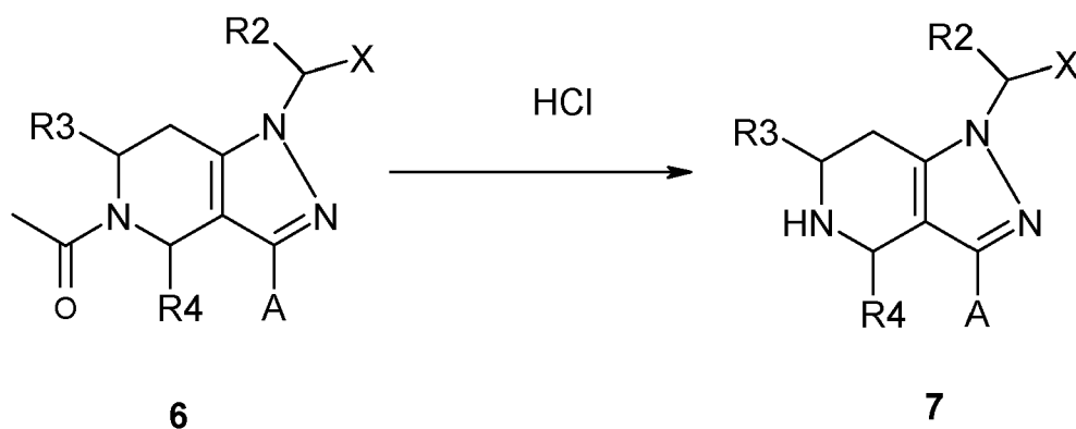
Scheme 5
