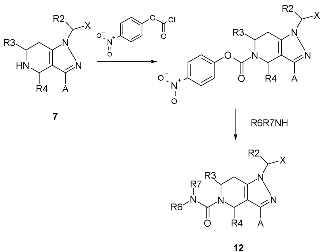
Scheme 9
