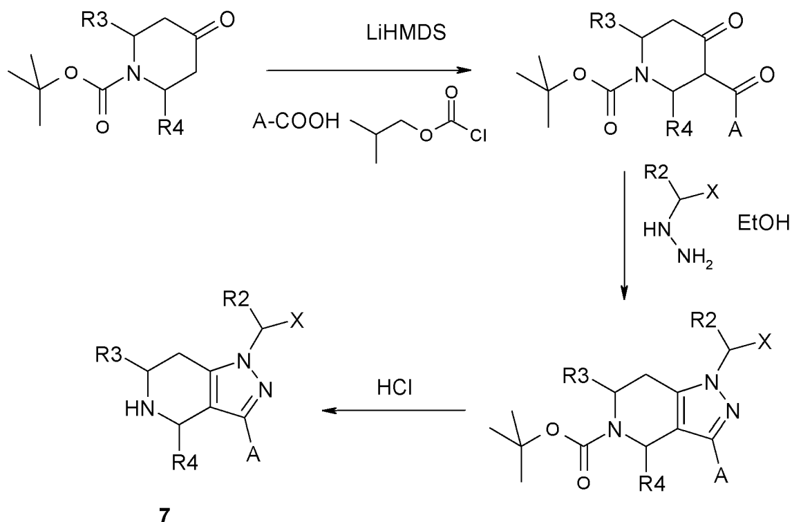
Scheme 4
