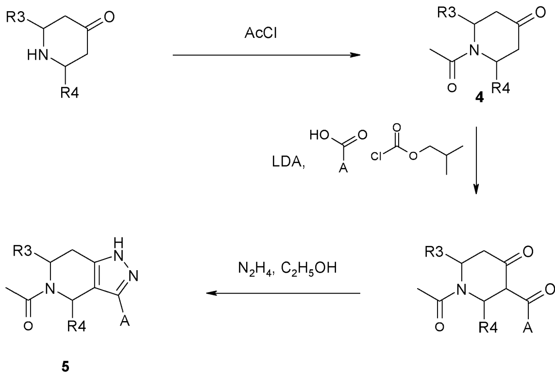
Scheme 2
