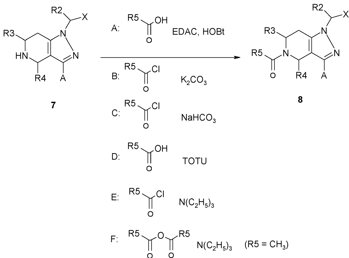
Scheme 6
