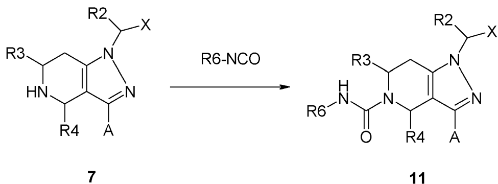
Scheme 8
