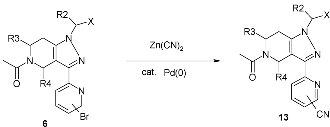
5 Scheme 10
