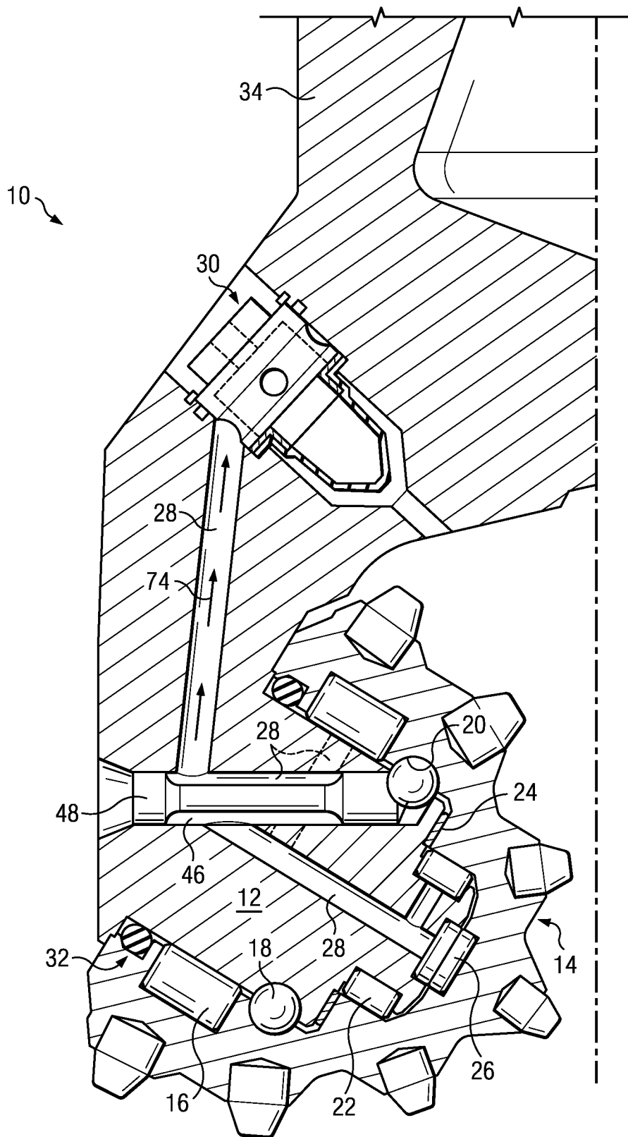
FIG. 1 (PRIOR ART)
