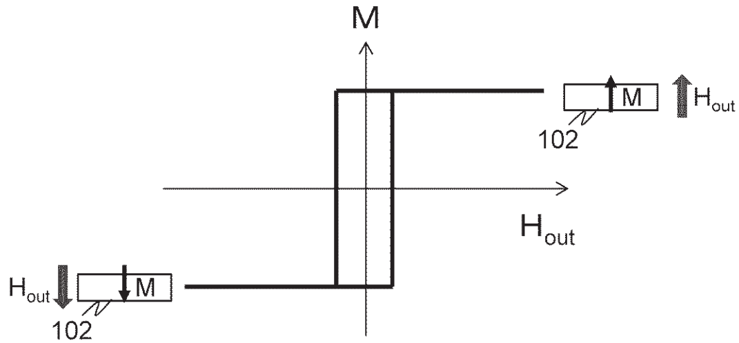
(1) PERPENDICULAR MAGNETIZATION FILM: SOLID FILM
