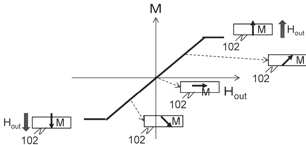
(2) PERPENDICULAR MAGNETIZATION FILM: AFTER CO/NH 3 PROCESSING
