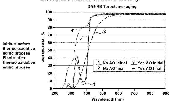
Excel chart Thermo oxidative stability
