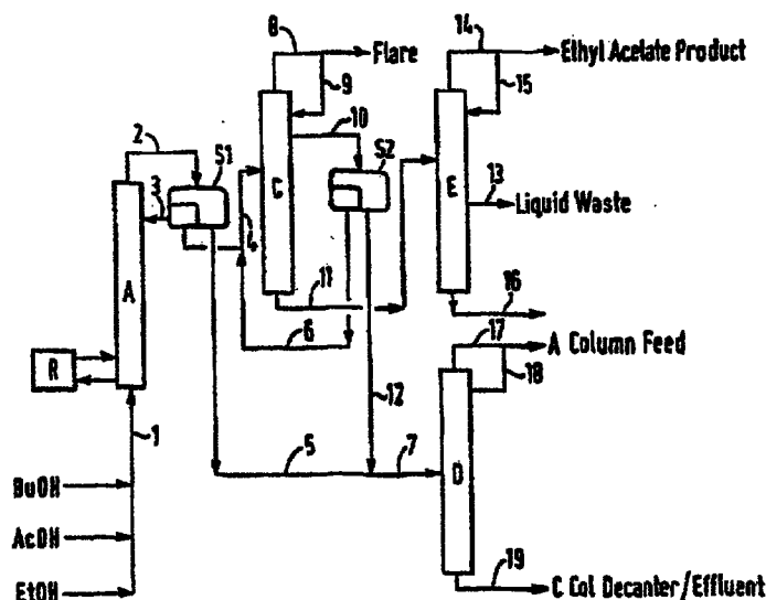
Coproduction: Proposed Distillation Layout (Resin Beds not Included)
